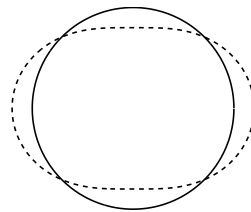
Fig. 2. Example of a 2-order ( m = 2 ) rotating force wave coming from the Fourier series development of radial air-gap Maxwell forces distribution. The fundamental difference with the deflection shape of the stator elliptical mode in Fig. 1 is the fact that the exciting force nodes are rotating, whereas the mode deflection nodes are steady, fixed according to the maximal stiffness points of the structure.
