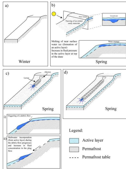
Figure 2: Scenario for the formation of debris flows during high obliquity period on the Russell dune.
