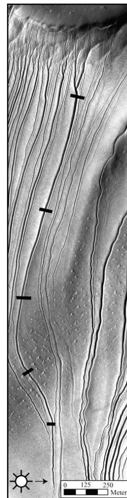
Figure 1: Position of the five cross sections studied along the gully. HiRISE image PSP_007229_1255 on the left. Image credits NASA/JPL/University of Arizona.
