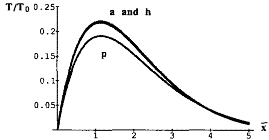
FIG. 9. As Fig. 8, \bar{\omega} = 1 .
