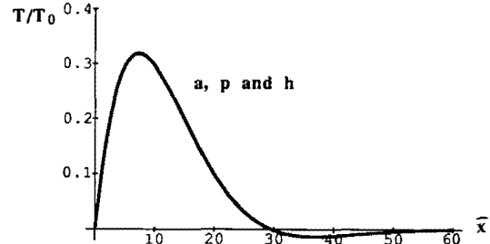
FIG. 8. Temperature profile in a semi-infinite bilaminated composite ( n = 0.9 ) subjected to a cosinusoidal temperature variation at the origin, for the dimensionless pulsation \bar{\omega} = 0.02 . h : homogenization; p : phenomenological approach; a : approximation.
