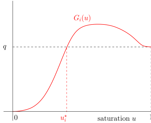
FIGURE 4. An example of function G_i fulfilling the assumptions (H5) . The represented value u_i^* defined in (H8) separates the values of the saturation where both phases flow in the same direction and the values of the saturation where both phases flow in opposite directions (cf. Remark 7).
