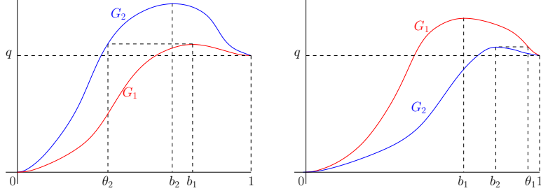
FIGURE 3. Example of functions G_i satisfying (H5) and of the so-called optimal connections \kappa_{\text{opt}}(x) (see [2, 8]).
