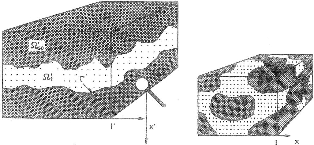
Fig. 2. Fractured medium periodic cell
