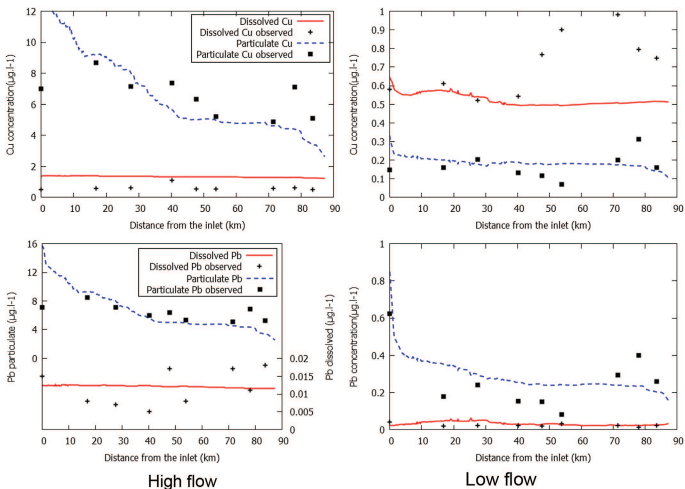
Fig. 5. Profile of the TMs concentration along the river. The top figures refer to Cu while the bottom figures refer to Pb. The profiles at the left are the simulations and observations made during the high flow ( 800 \text{ m}^3 \text{ s}^{-1} ) of 18 May 2005. The profiles at the right are the simulations (this study) and observations (Aubert et al., unpublished data) made during the low flow ( 80 \text{ m}^3 \text{ s}^{-1} ) of 10 October 2005. The observations were made at Portet (at the inlet) and at the eight sampling stations (G1 to G8).
