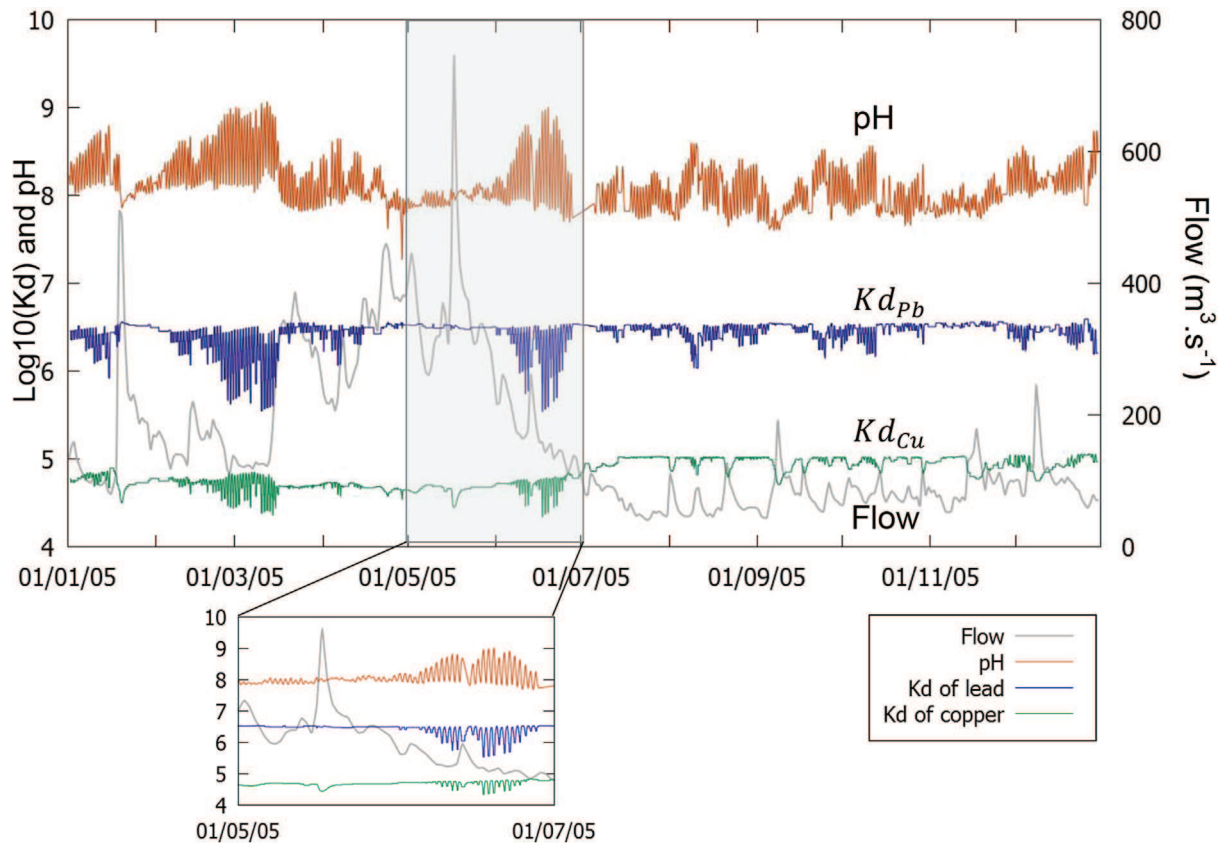
Fig. 6. Variation of the simulated K_d of Cu (A) and Pb (B) under variable hydrological conditions during the year 2005. The K_d was calculated at the sampling point G5 (54 km after the inlet). The K_d is presented with the flow and the observed pH in the river. A zoom is provided over the high flow of May and the following diurnal cycles.
