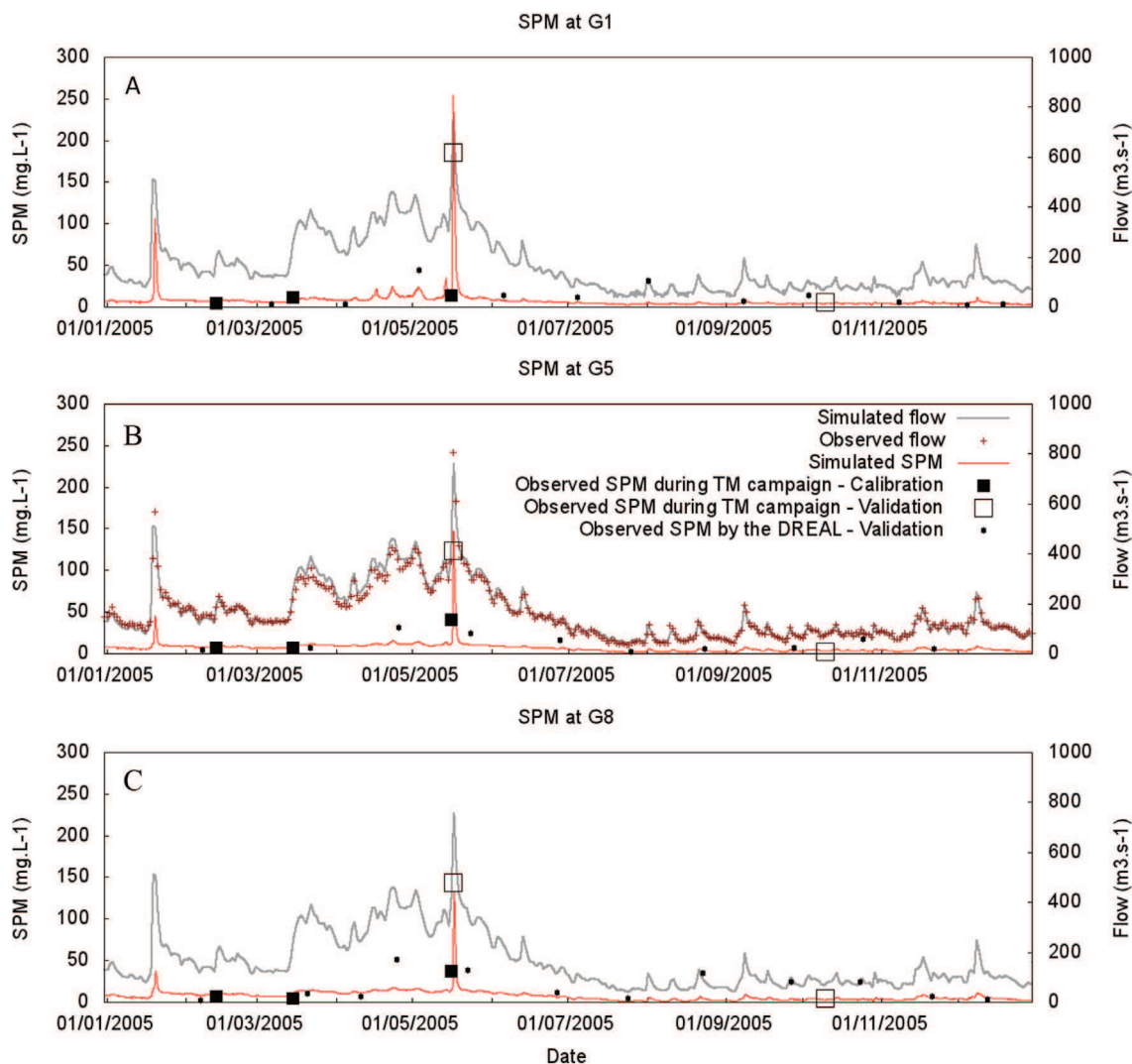
Fig. 2. The simulated trends of SPM and discharge are shown for sampling point G1 (A), G5 (B) and G8 (C) (see Fig. 1) for the year 2005. The observed SPM refer to the sampling campaigns while the observed SPM DREAL are relative to data collected by the water agency DREAL (see section 2.6.3). The observed flows are presented at G5 (dotted) with the simulated flow to validate the hydrodynamic model. There are 27 km from the inlet of the model to point G1, 54 km to the sampling point G5 and 83 km to the sampling point G8.
