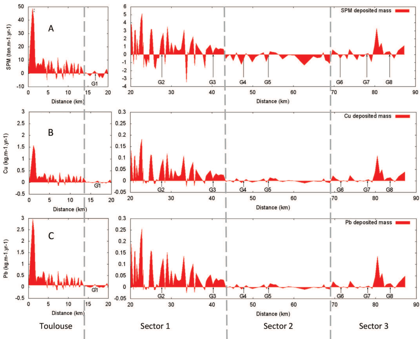
Fig. 8. Accumulated (positive) or eroded (negative) mass of SPM (A), Cu (B) and Pb (C) along the river profile over the year 2005, according to the MOHID – WHAM model. The sampling points (from G1 to G8) are indicated. The river exits the city of Toulouse after 14 km where high sedimentation rates are simulated. Therefore, the scale is different before and after the city (left diagrams). The alluvial plain is further decomposed in three sectors exhibiting different behaviors (sectors 1 to 3).
