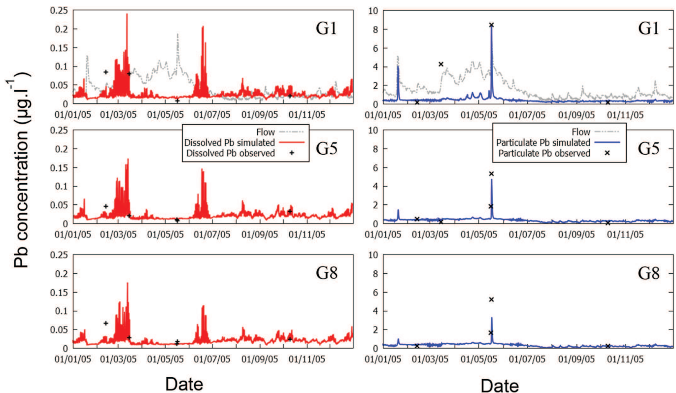
Fig. 4. Annual Variation of simulated Pb concentration in the dissolved (left) and particulate (right) phase at the three sampling points G1, G5 and G8 (top right corner, see Fig. 1) during the year 2005. The observations (Aubert et al., unpublished data) collected during the four sampling campaigns are identified by crosses. The simulated flow at the first sampling point (G1) is shown to provide the hydrological context of the data.
