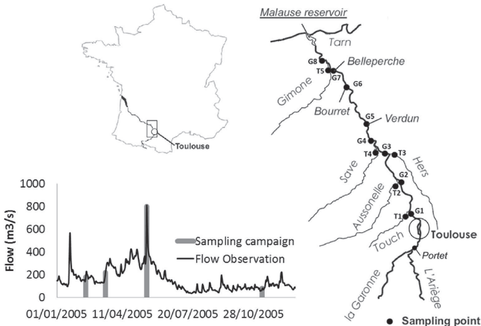
Fig. 1. The Garonne River study site in the South-West of France. The model was applied over the Garonne river section between Portet (upstream Toulouse city) and station G8 (upstream the Malause reservoir before the confluence with the Tarn river) for a total reach of 87 km. The sampling sites in Garonne main channel are indicated by “Gx” symbols and the tributaries sampled by “Tx” symbols. The hydrology of the sampling campaigns is also represented and was observed at the sampling point G5.
