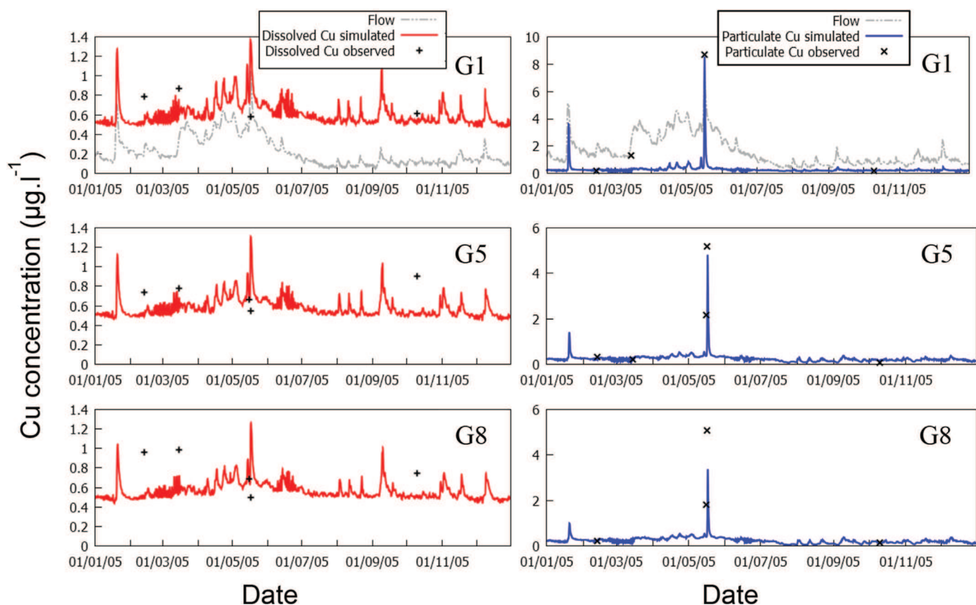
Fig. 3. Annual Variation of simulated Cu concentration in the dissolved (left) and particulate (right) phases at three sampling points G1, G5 and G8 (top right corner, see Fig. 1) during the year 2005. The observations (Aubert et al., unpublished data) collected during the four sampling campaigns are identified by crosses. The simulated flow at the first sampling point (G1) is shown to provide the hydrological context of the data.
