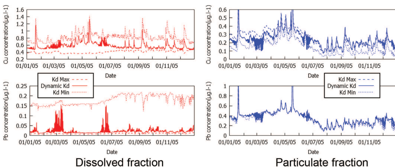
Fig. 7. Comparison of dissolved (left) and particulate concentrations (right) for Cu (up) and Pb (down) at the sampling point G5 simulated by the dynamic MOHID – WHAM model with the constant K_d model of sorption. Two K_d have been used: the maximum and the minimum K_d observed during the sampling campaign (see Table 5). The figure does not show the maximal concentration of January and May high flows as all three scenarios presented a mismatch of less than 5% during these two events.
