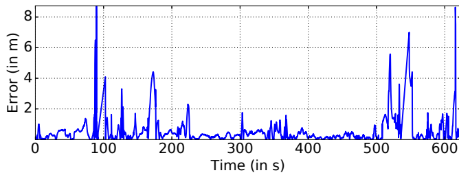
Figure 12. GNSS error during the test. Spikes are clearly visible, corresponding areas with poor GNSS reception (high-rise buildings nearby).
