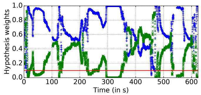
Figure 10. Evolution of the weights of hypotheses. The blue curve (“+” signs) is the correct matching. For most of the time it is the most likely hypothesis. The red line denotes a 0.1 weight threshold.
