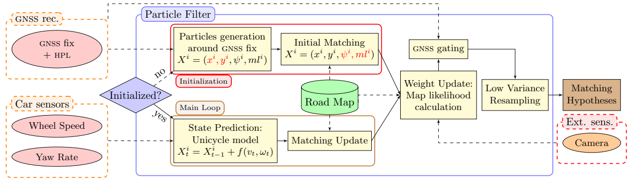
Figure 2. Flowchart of the map-matching process. Based on a particle filter, the algorithm takes as input a GNSS fix with HPL and the car’s dead-reckoning. The process is separated into two steps, namely a computationally intensive initialization followed by a highly efficient main loop. Exteroceptive information is used in the computation of likelihood.
