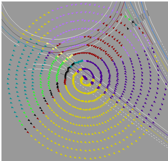
Figure 3. Particle Initialization: colors denote the matched link. The initial heading corresponds to the matched link. Some particles are far from the links due to the 50 m HPL (high value chosen to be conservative), but will potentially be quickly eliminated during a resampling step.
