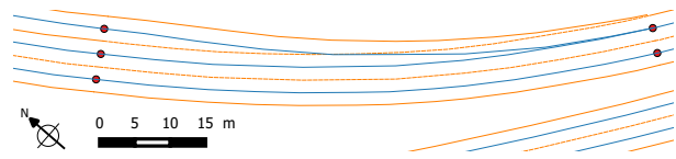
Figure 1. Detail of the map at a lane forking in Compiègne, France. The centerlines of the lanes are drawn in blue and the lane markings in brown. The upper road is drivable from east to west. The upper blue polyline of the right lane separates into two lanes.
