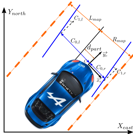
Figure 7. Reference frames used by the camera for describing lane markings. Dashed orange lines represent lane marking data from the map. Camera detections are represented in blue. The lane centerline is in black.
