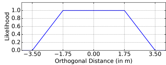
Figure 6. Trapezoidal likelihood function for orthogonal distance (based on the French regulations relating to the width of roads). The car is equally likely to be in any lateral position on the roadway.
