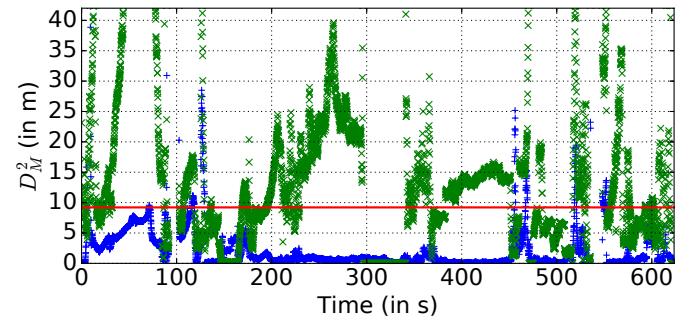
Figure 11. Squared Mahalanobis distances for the matching hypotheses (the correct hypothesis shown as blue “+”). The red line denotes the critical value for p_{fa} = 0.01 .
