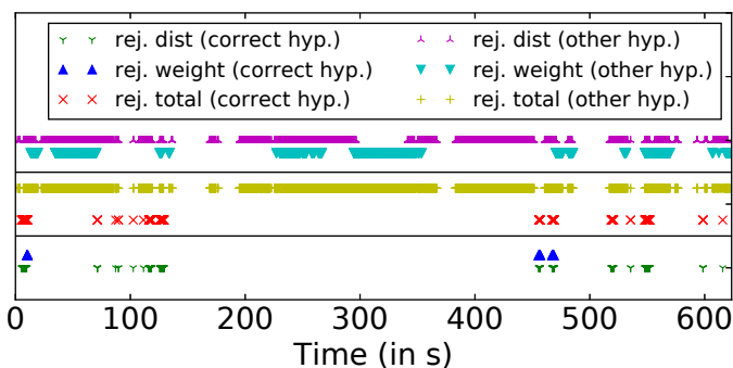
Figure 14. Rejection classification by cause, for the correct matching and the others. A point indicates that the corresponding hypothesis was rejected at this time step for the given reason.
