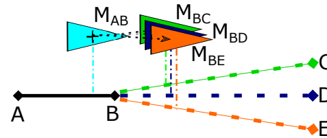
Figure 5. Lane bifurcation where particle cloning occurs: the particle M_{AB} is duplicated into M_{BC} , M_{BE} and M_{BD} in order to do a thorough search.
