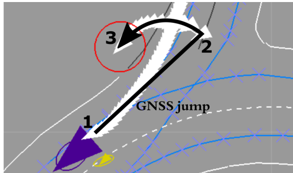
Figure 13. Screenshot of the situation at t = 127 s. A biased GNSS position causes the two matching hypotheses to be rejected.
