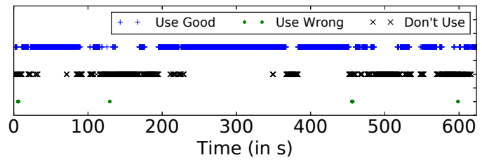
Figure 15. “Use/Don’t Use” decisions by the integrity monitoring method. It can be seen that misdetections (“Use Wrong”) are rare. Positioning availability corresponds to “Use Good”.
