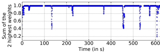
Figure 9. The sum of two highest weights. 95% of the time the sum is higher than 0.95. When more hypotheses are present, they are quickly eliminated (in the order of 10 seconds)
