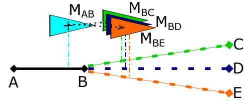
Figure 5. Lane bifurcation where particle cloning occurs: the particle M_{AB} is duplicated into M_{BC} , M_{BE} and M_{BD} in order to do a thorough search.
