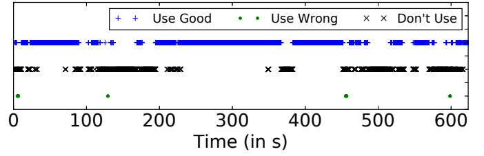
Figure 15. “Use/Don’t Use” decisions by the integrity monitoring method. It can be seen that misdetections (“Use Wrong”) are rare. Positioning availability corresponds to “Use Good”.
