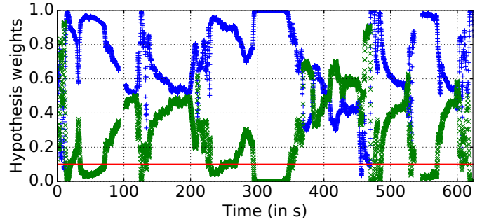
Figure 10. Evolution of the weights of hypotheses. The blue curve (“+” signs) is the correct matching. For most of the time it is the most likely hypothesis. The red line denotes a 0.1 weight threshold.
