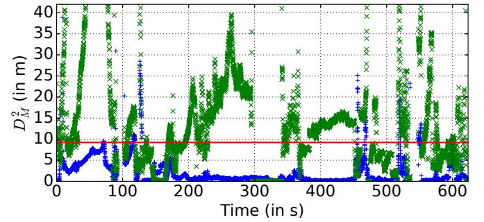
Figure 11. Squared Mahalanobis distances for the matching hypotheses (the correct hypothesis shown as blue “+”). The red line denotes the critical value for p_{fa} = 0.01 .
