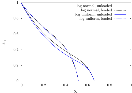
Figure 3: Estimates of gas relative permeabilities without loading (line) and with loading (dashes) for \phi = 0.1 and \Delta\phi = 0.03
