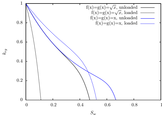
Figure 4: Estimates of gas relative permeabilities : effect of the laws f and g , for a log-uniform p.d.f. \alpha with a standard deviation of 1, \phi = 0.1 and \Delta\phi = 0.03 .
