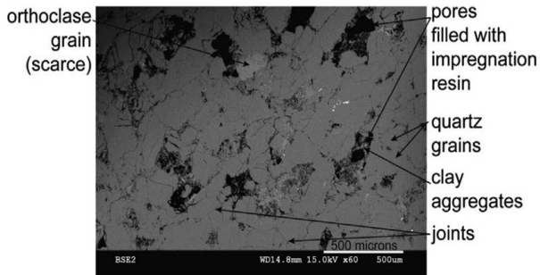
Figure 2: SEM image of a tight sandstone
