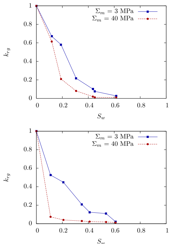
Figure 1: Gas relative permeability measurements for 2 low permeable sandstone samples - loading of 3MPa (blue curve) - 40 MPa (red curve)
