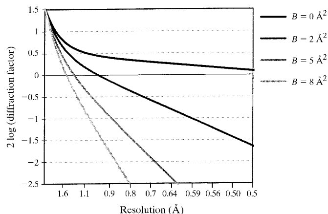
Figure 4 Diffraction power of a C atom as a function of resolution for several isotropic temperature factors. The square of the scattering factor has been chosen as it is closely related to the measured diffraction intensities (after Lorentz polarization correction).
