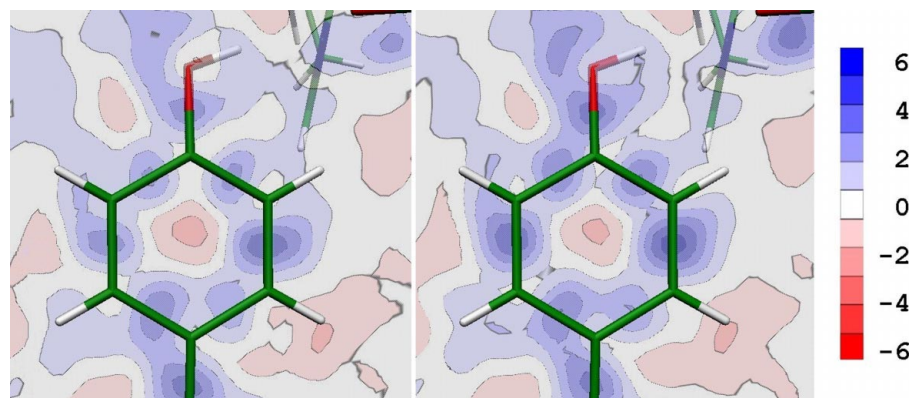
Figure 12 Residual electron-density map ( F_{\text{obs}} - F_{\text{cal}} ) of aldose reductase in the aromatic plane of residue tyrosine 48. Left: after classical refinement. Right: after high-order refinement.
