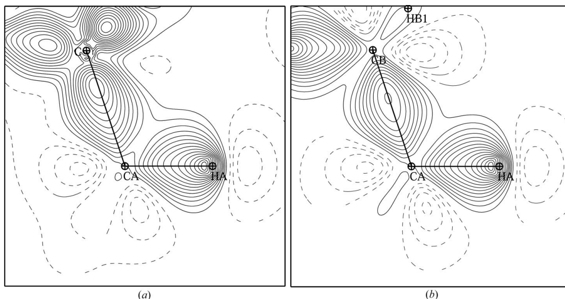
Figure 10 Deformation of the static electron density in the C\alpha - H\alpha -C and C\alpha - H\alpha - C\beta planes of the polypeptide refined versus the diffraction data of protein crambin (Jelsch et al. , 2000). Contours \pm 0.05 \text{ e \AA}^{-3} , black lines \delta\rho > 0 , grey dotted lines \delta\rho < 0 .
