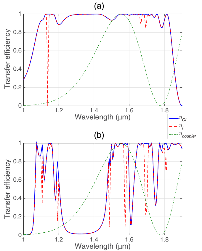
FIG. 6. Evolution of the transfer efficiencies with wavelength for (a) N = 3 and (b) N = 6 . The refractive index profiles correspond to the ones of Fig. 1. \eta_{CI} ( \eta_I ) is the transfer efficiency for the counterintuitive case (the intuitive case). The efficiency spectrum is compared to the one of a directional coupler ( \eta_{coupler} ) composed of two straight waveguides and tuned to a wavelength of 1.55 \mu\text{m} (see text).
