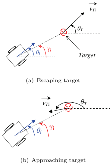
Figure 5: Escaping/Approaching target.
