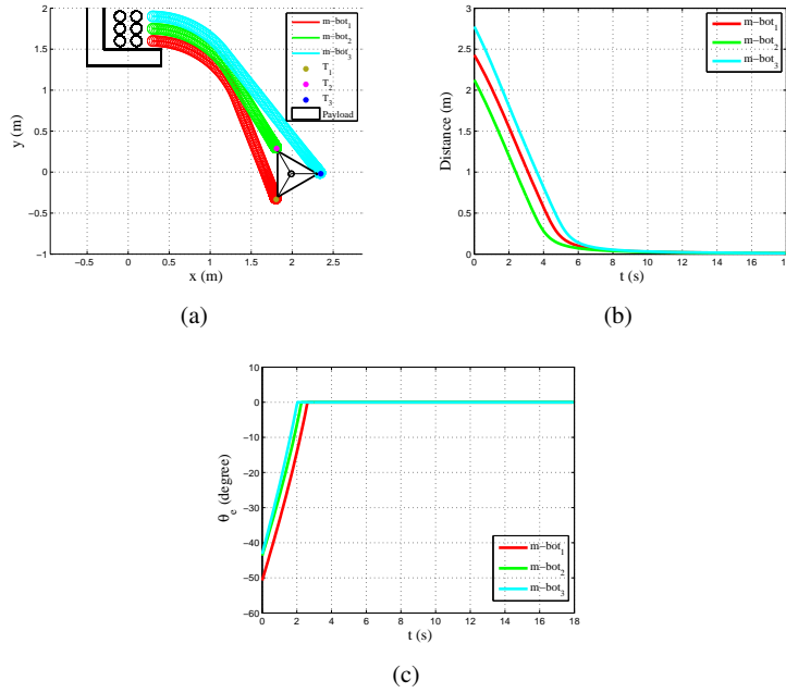
Fig. 7 M-bots target reaching (TR): a) Trajectories of the m-bots reaching the desired positions; b) Position error for TR; c) Angle Error for TR.
