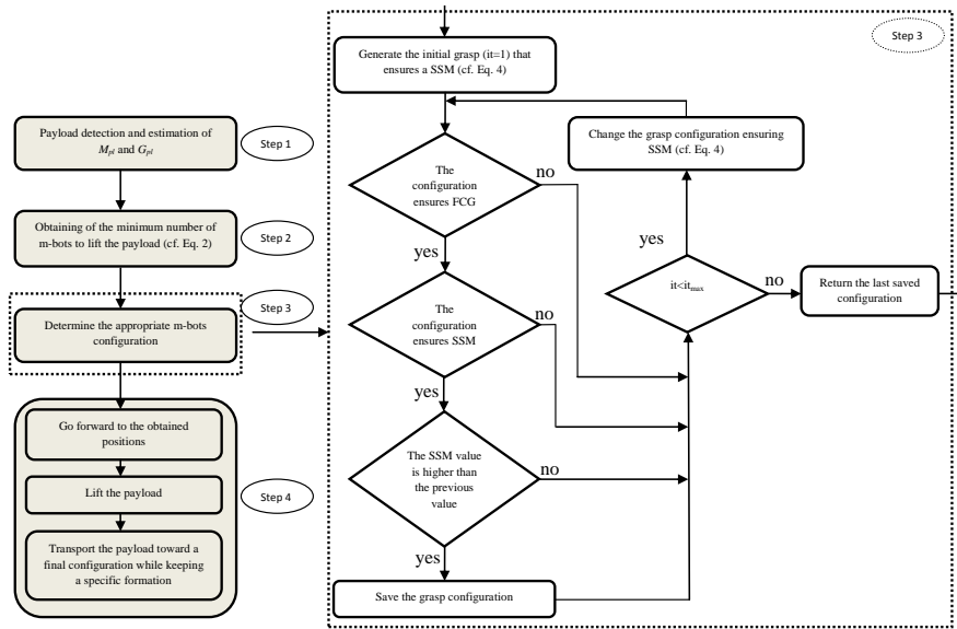
Fig. 2 Flowchart for co-manipulation with C 3 Bots
