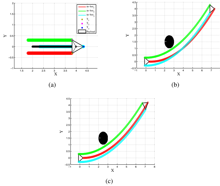
Fig. 8 Virtual structure (VS) navigation: a) The p-bot is navigating as a rigid Virtual Structure (VS); b) The p-bot avoids the obstacle and keeps the same orientation; c) The p-bot avoids obstacle and changes the payload orientation.
