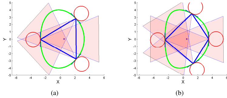
Fig. 5 Simulation results: a) 3 m-bots positioning; b) 4 m-bots positioning
