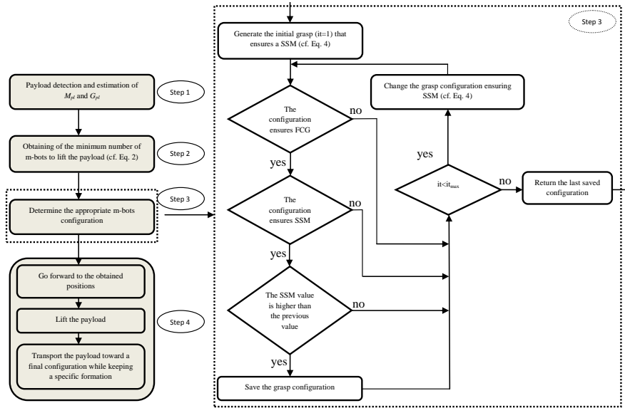
Fig. 2 Flowchart for co-manipulation with C 3 Bots
