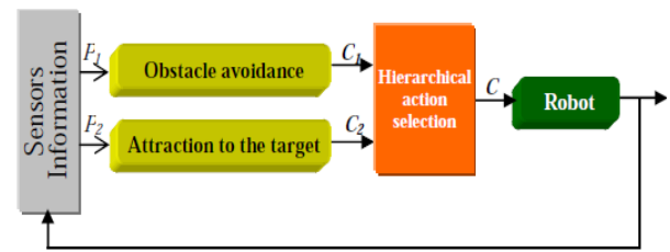
Fig. 2. Control architecture for mobile robot navigation [12]
