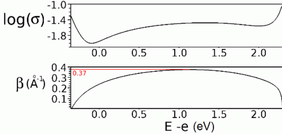
Figure 4. In the lower part, the decay parameter obtained by linear regression as a function of E - e for E in the electronic gap of the molecular wire figure 2. the 30 electrons of the molecular wire are frozen in their HF ground state. In the upper part, the standard deviation for each data set.
