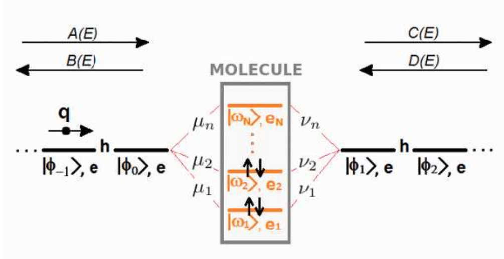
Figure 1. Model of the molecular junction used for the CI-ESQC calculations. The electrodes are empty except for the incident or the scattered particle q (electron or hole). The molecule is represented by its molecular orbitals (MO) occupied by m electrons not frozen in a particular electronic configuration during the scattering process.
