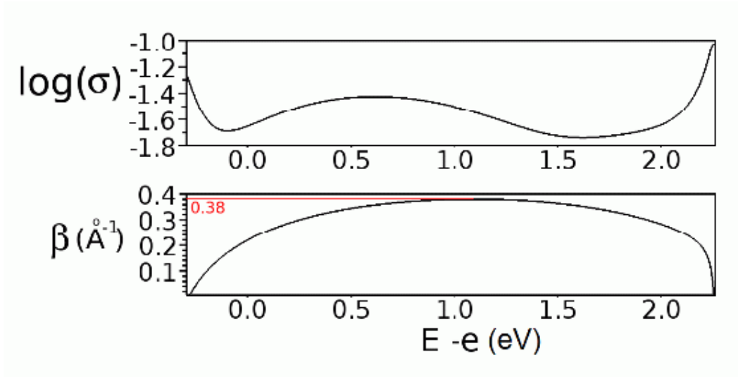
Figure 6. In the lower part, the decay parameter obtained by linear regression as a function of E - e for E in the electronic HOMO-LUMO gap of the molecular wire figure 2. Here, the active space is constructed starting from 6 MOs occupied by 6 electrons with the excitations limited to the mono and bi excitations. In the upper part, the standard deviation for each data set.
