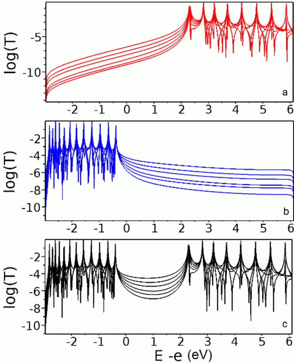
Figure 3. The T(E) transmission coefficients for different molecular wire lengths N_l = [10, 12, 14, 16, 18, 20] as a function of E - e for the molecular junction figure 2 with N = 30 . Here, the 30 electrons of the molecular wire are frozen in their HF ground state. In (a), the scattered particle is an electron, in (b), a hole and in (c), the system is in a coherent superposition between an electron and a hole scattering states.
