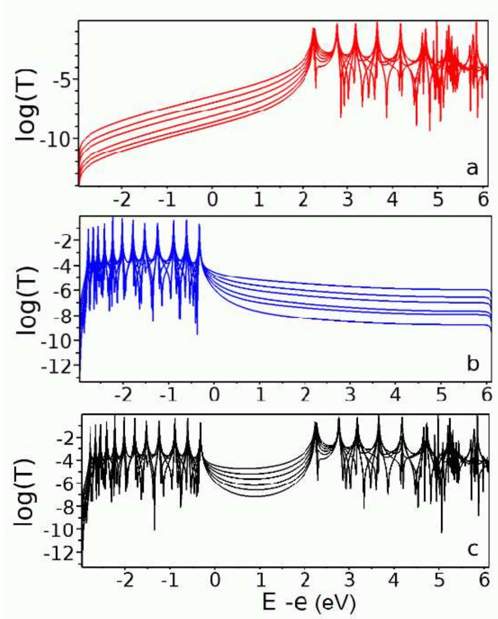
Figure 5. The T(E) transmission coefficients for different molecular wire lengths N_l = [10, 12, 14, 16, 18, 20] as a function of E - e for the molecular junction figure 2 with N = 30 . Here, the active space is constructed starting from 6 MOs occupied by 6 electrons with the excitations limited to the mono and bi excitations. In (a), the scattered particle is an electron, in (b), a hole, and in c the system is in a coherent superposition between an electron and a hole scattering state.
