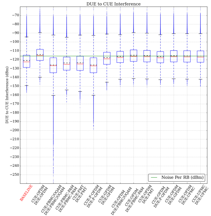
Fig. 6. The DUE to CUE interference is similar to the value of noise per resource block for coexistence cases.
