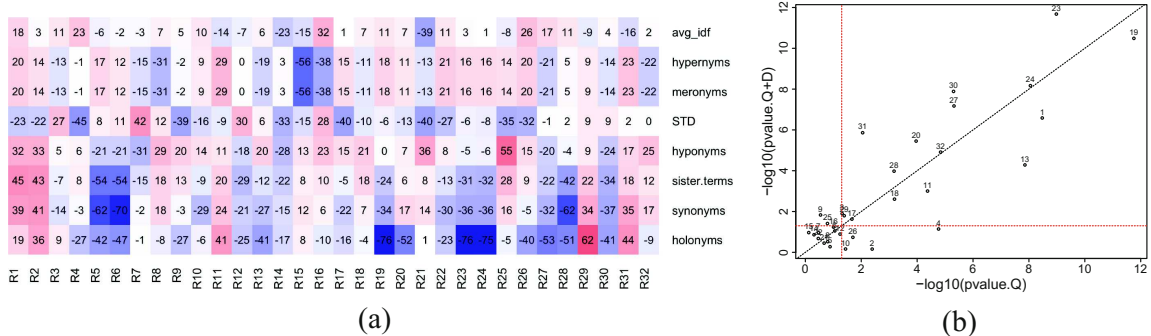
Fig. 1. (a) Correlations (x100) between reasons (X axis) and query features and automatic predictors (Y axis) when using Q. (b) Significance of the correlations between reasons and predicted difficulty (Q on X axis and Q+D on Y Axis). (Color figure online)
