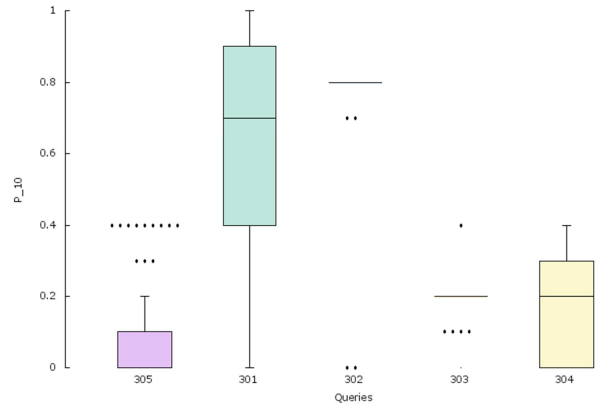
Fig. 5. Boxplots for the 5 queries with the most reformulations with respect to P10 (sorted by descending order of the number of reformulations made by players).
