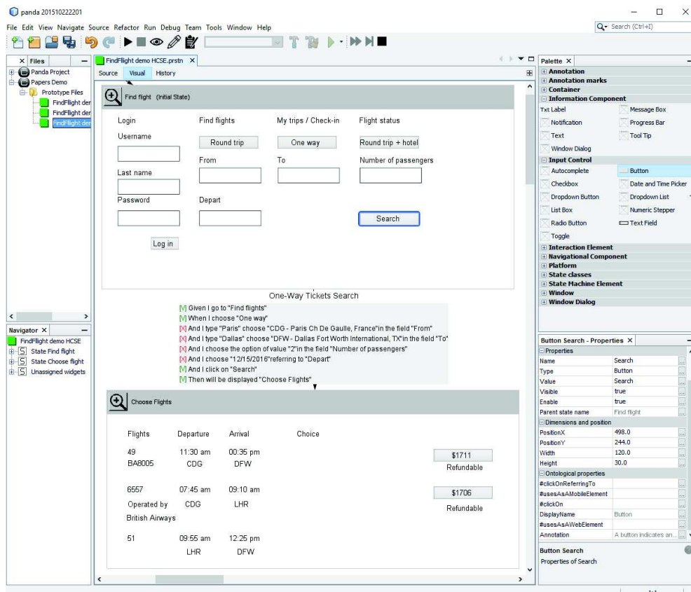
Figure 23. PANDA screenshot
