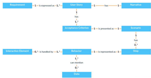
Fig. 2. Conceptual Model for testable requirements
