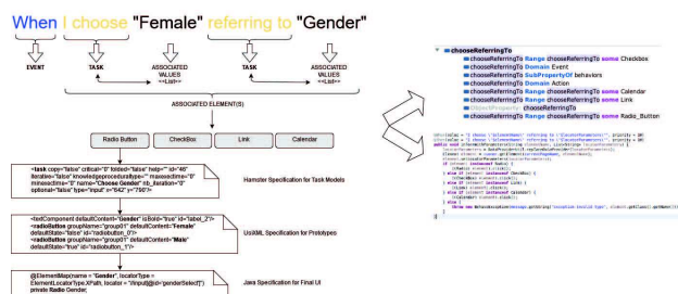
Fig. 3. Identifying behaviors through multiple artifacts
