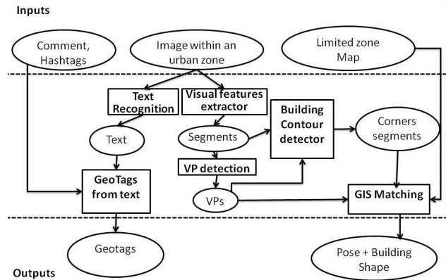
Figure 3. Features extraction layer.
