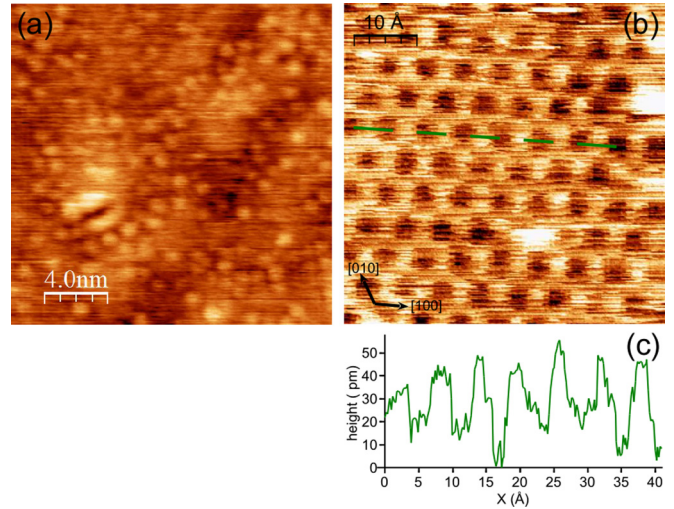
FIG. 2. NC-AFM topography image of AlN(0001) surface after growth of a 200-nm-thick sample at T_{\text{substrate}} = 950^\circ \text{C} , \text{BEP}_{\text{NH}_3} = 10^{-5} Torr and a growth rate of 100 nm/h (a), and 5 nm thick at 10 nm/h (b). (c) Cross section along the dashed line in (b). NC-AFM parameters: (a) A = 5 \text{ nm} , \Delta f = -65 \text{ Hz} , f_0 = 278.4 \text{ kHz} , Q = 35\,255 , U_{\text{sample}} = -4.7 \text{ V} ; (b) A = 8 \text{ nm} , \Delta f = -25 \text{ Hz} , f_0 = 274.8 \text{ kHz} , Q = 42\,780 , U_{\text{sample}} = -1 \text{ V} .
