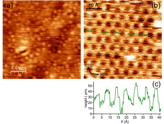
FIG. 2. NC-AFM topography image of AlN(0001) surface after growth of a 200-nm-thick sample at T_{\text{substrate}} = 950^\circ\text{C} , \text{BEP}_{\text{NH}_3} = 10^{-5} Torr and a growth rate of 100 nm/h (a), and 5 nm thick at 10 nm/h (b). (c) Cross section along the dashed line in (b). NC-AFM parameters: (a) A = 5 \text{ nm} , \Delta f = -65 \text{ Hz} , f_0 = 278.4 \text{ kHz} , Q = 35\,255 , U_{\text{sample}} = -4.7 \text{ V} ; (b) A = 8 \text{ nm} , \Delta f = -25 \text{ Hz} , f_0 = 274.8 \text{ kHz} , Q = 42\,780 , U_{\text{sample}} = -1 \text{ V} .
