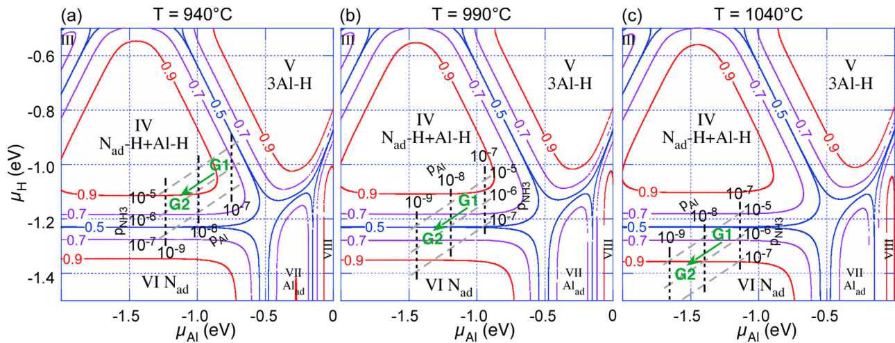
FIG. 4. Phase diagrams with changing temperature: (a) 940° C, (b) 990° C, and (c) 1040° C. The isoconcentration curves are blue, purple, and red for c_i = 0.5, 0.7, and 0.9, respectively. The chemical potentials ( \mu_{Al}, \mu_H ) are plotted for three isopressures of p_{Al} (black dotted line) and p_{NH_3} (gray dashed line). The beginning and the end of the green arrows indicate the change in chemical potential when passing from G1 to G2 growth conditions.
