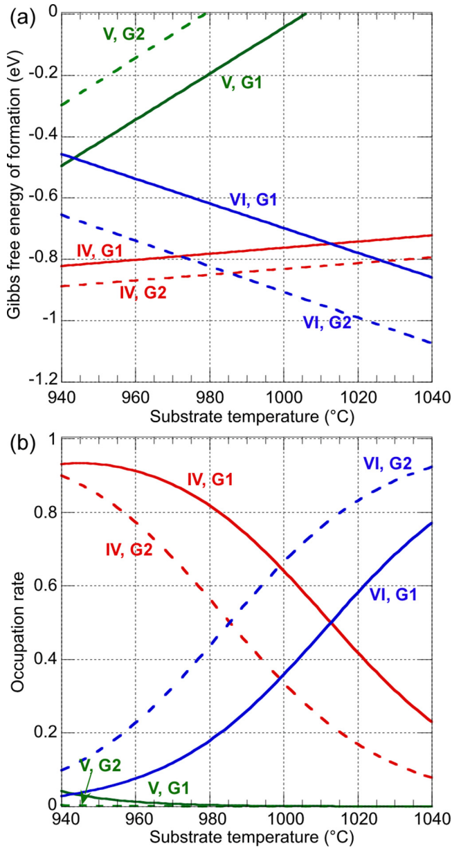
FIG. 3. (a) Gibbs free energy of formation vs substrate temperature for the three reconstructions IV( N_{ad} -H+Al-H), V(3Al-H), and VI( N_{ad} ) calculated with the experimental pressures p_{NH_3} = 2 \times 10^{-6} Torr and p_{Al} = 3 \times 10^{-8} Torr, and 3 \times 10^{-9} Torr corresponding to the growth rate G1 and G2, respectively. (b) Occupation rate calculated with the Boltzmann distribution for the three reconstructions and the two sets of growth G1 and G2.
