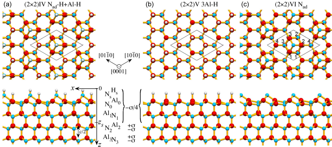
FIG. 1. Top and side views along the [1\bar{1}00] axis of the atomic models of the three (2 \times 2) reconstructions, N_{ad} -H+Al-H, 3Al-H, and N_{ad} obtained by DFT. The (2 \times 2) unit cell appears on the top views as a black lozenge. Al, N, and H atoms are represented as red, blue, and white balls, respectively.
