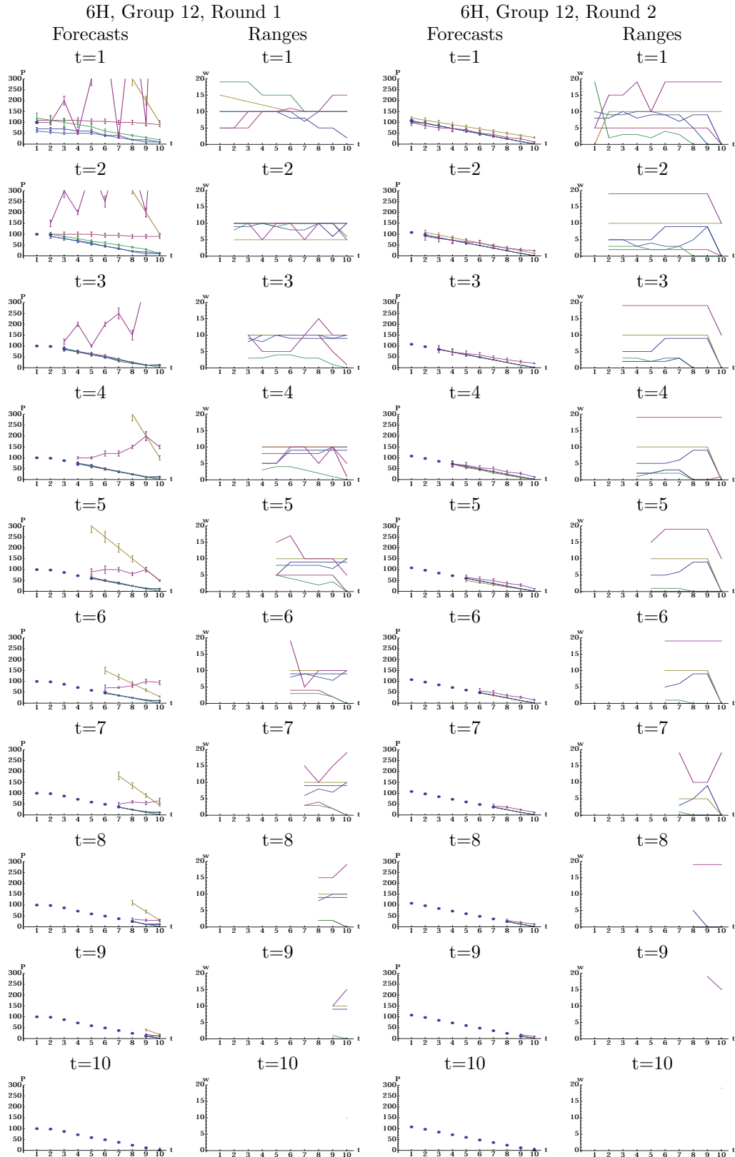
Figure 4: Dynamics of forecasts and prices observed in Group 12 of 6H treatment (thin lines: individual traders, dots: realized prices).
