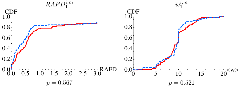
Figure 1: Cumulative distribution of RAFD_1 (left) and \bar{w}_1 (right) in the 6H (solid red line) and 1H5C (dashed blue line) treatments in period 1 of Round 1. P-values are from the two-sample permutation test (two-tailed).
