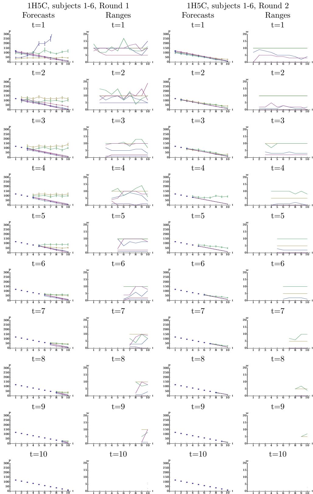
Figure 5: Dynamics of forecasts and prices observed for Subject 1 to 6 in 1H5C treatment (thin lines: individual traders, dots: realized prices). 14
