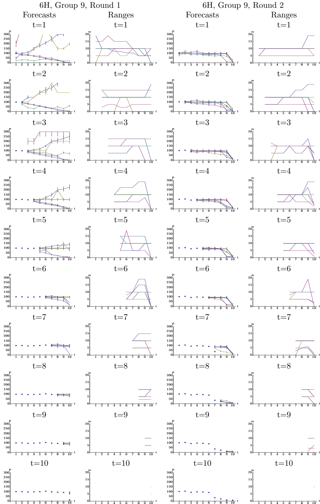
Figure 3: Dynamics of forecasts and prices observed in Group 9 of 6H treatment (thin lines: individual traders, dots: realized prices).
