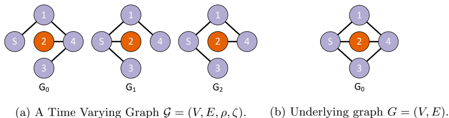
Fig. 1: Example of a simple TVG and its underlying static graph.
