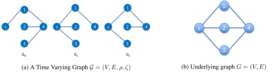
Figure 3: Example of a simple TVG and its underlying static graph.
