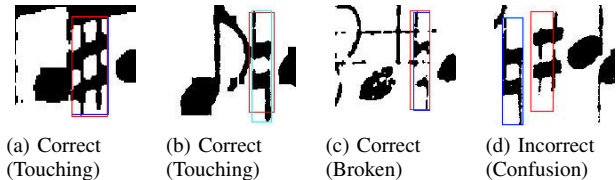
Fig. 1. Correct and incorrect detection of accidentals using in parallel the best classification and localization models. Red boxes are predictions and blue boxes are ground-truth.
