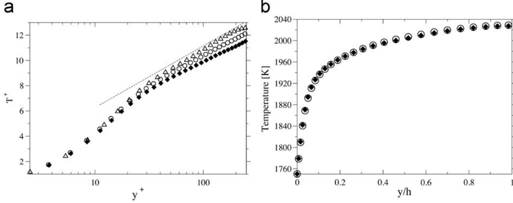
Fig. 5. Left: mean temperature in wall units. Right: mean temperature profile across the channel. Three simulations are represented by the following symbols: \triangle , non-reactive simulation without radiation; \circ , multicomponent simulation without radiation; \blacklozenge , coupled multicomponent simulation with radiation; --- , Kader logarithmic law for Re \rightarrow \infty .
