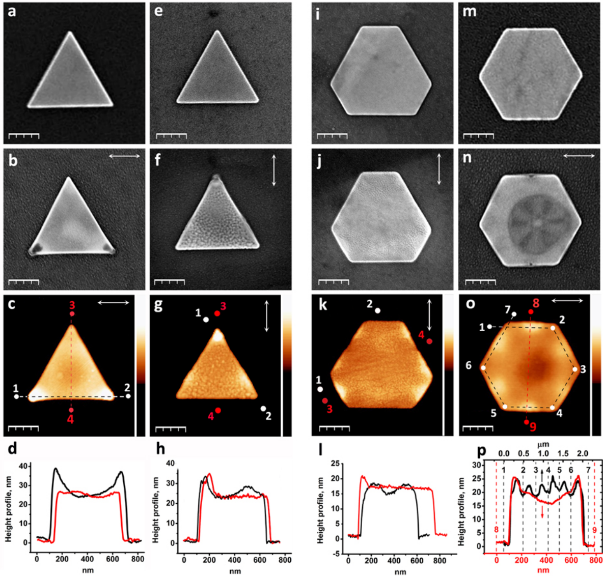
Figure 2. (a, b) SEM images of a sharp triangular Au prism (a) before and (b) after pulsed laser irradiation with horizontally polarized laser beam. (e, f) SEM images of another Au prism (e) before and (f) after irradiation with vertically polarized laser beam. The polarization direction is indicated by the double headed arrows. (c, g) AFM micrographs of the Au prisms after their respective irradiation, (d, h) Height profiles along the segments 1-2 (black line) and 3-4 (red line) marked in the panels (c) and (g). (i, m) SEM images of (i) a truncated triangular and (m) a hexagonal Au prisms before irradiation. (j, n) SEM images of the same Au prisms after irradiation. (k, o) AFM micrographs, corresponding to panels (j,n). (l, p) AFM height profiles along the segments 1-2 or 1-7 (black lines)
