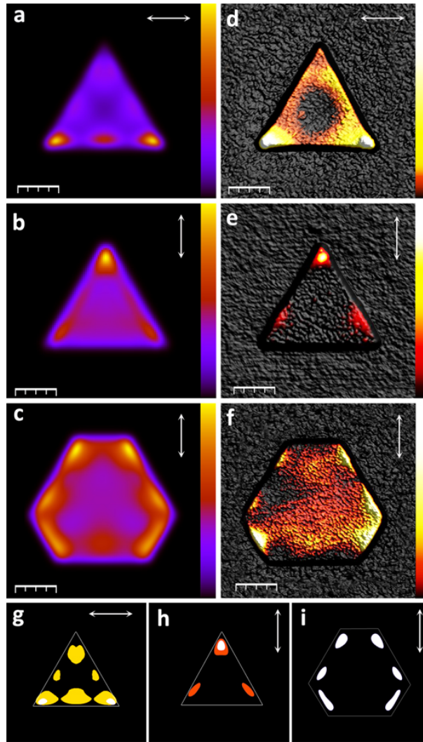
Figure 4. (a-c) Calculated partial SP-LDOS of (a,b) triangular and (c) truncated platelets projected along the direction shown by the double-headed arrows. The excitation wavelength is 800 nm. Each SP-LDOS map is normalized to its maximal value. (d-f) AFM images of prisms after irradiations at 800 nm. Laser polarization directions are indicated by the white double-headed arrows. (g-i) Thresholded calculated partial SP-LDOS from the panels (a-c), respectively. In (g) yellow color depicts regions where the normalized partial SP-LDOS in panel (a) exceeds 50%. In (h), orange shows the areas in (b) where the normalized SP-LDOS exceeds 60%. In (g-i), white areas corresponds to a normalized SP-LDOS exceeding 75% in (a-c). Scale bars are 200nm.
