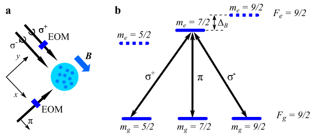
Figure 1. Tripod scheme. a , laser beams polarizations and propagation directions along a magnetic bias field \mathbf{B} . Two EOMs are used to sweep the two independent relative phases of the laser beams. b , bare energy level structure of the tripod scheme, implemented on the intercombination line of Strontium-87. The magnetic bias field shifts consecutive excited levels by \Delta_B \simeq 760\Gamma = 5.7 MHz. It allows each tripod polarized laser beam to selectively address one of the magnetic transitions marked by the black arrows.
