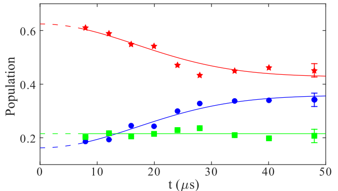
Figure 2. Ballistic expansion. Time evolution of the bare state populations after the tripod ignition sequence (duration t_0 \simeq 8 \mu\text{s} ) is completed and laser beams have reached equal Rabi frequencies \Omega = 2\pi \times 250 \text{ kHz} . The blue circles, the green squares, and the red stars correspond to the populations \bar{P}_1 , \bar{P}_2 , and \bar{P}_3 with |i\rangle \equiv |m_g = i + 3/2\rangle ( i = 1, 2, 3 ), respectively. Solid lines: theoretical predictions given by equations. 5. The temperature T , the initial and the final populations of each spin state are the fit parameters. The dashed lines, at early times, extrapolate the fits into the time window t_0 . We get a temperature T = 0.5(1) \mu\text{K} meaning that the atoms do not move significantly during the dark-state preparation sequence since \bar{v}t_0/\lambda \simeq 0.08 .
