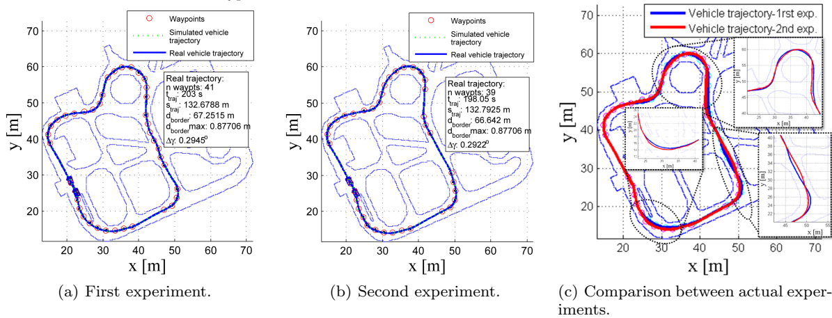
Fig. 25 Actual vehicle's trajectories for different obtained set of waypoints.
