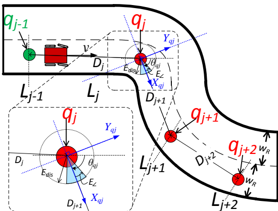
Fig. 3 Description of waypoints assignment.
