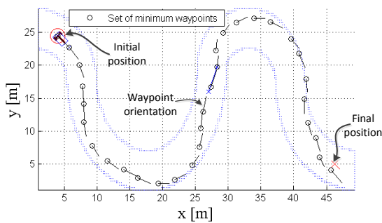
Fig. 17 Set of waypoints using probabilistic expanding tree.
