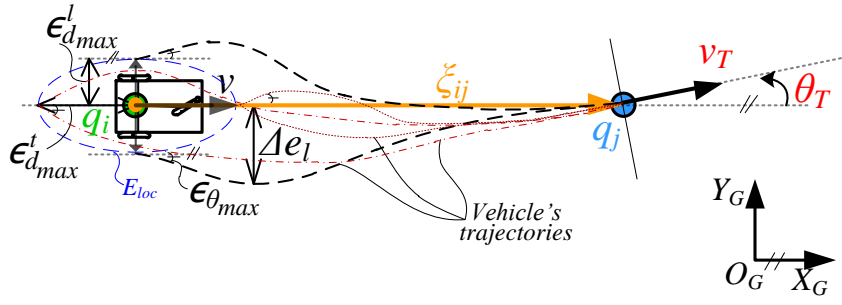
Fig. 10 Vehicle's trajectories which starts from extreme configurations ( \pm\epsilon_{d_{max}}^l , \pm\epsilon_{d_{max}}^t and \pm\epsilon_{\theta_{max}} ) in the localization uncertainties ellipse E_{loc} . \Delta e_l is the maximum lateral deviation of all vehicle trajectories.
