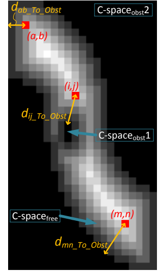
Fig. 7 Representation in gray scale w.r.t the distance to the closest C\text{-space}_{obst} (the whitest area represents the safest area).
