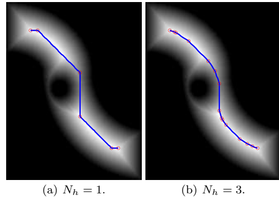
Fig. 9 Different sets of waypoints for different number of possible neighbor cells.
