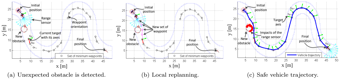
Fig. 21 Local replanning for unexpected obstacle.
