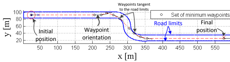
(a) Minimum set of waypoints for fastest trajectory.
