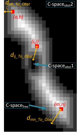
Fig. 7 Representation in gray scale w.r.t the distance to the closest C\text{-space}_{obst} (the whitest area represents the safest area).
