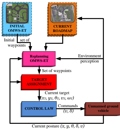
Fig. 20 Schema of the local replanning.
