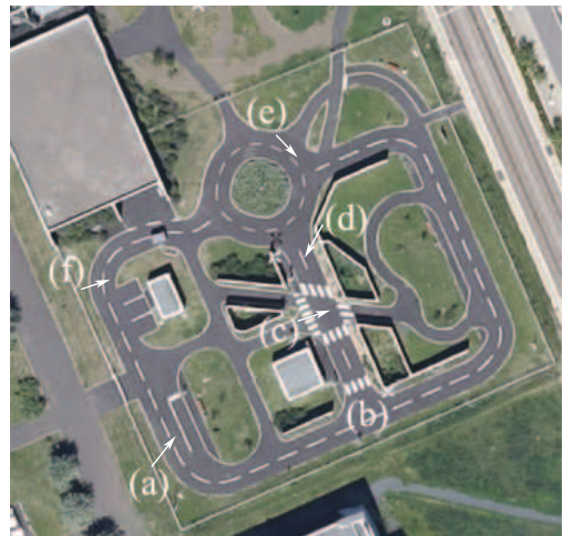
Figure 18: PAVIN experimental platform. (a) to (f) correspond to the locations shown in Fig. 19.
