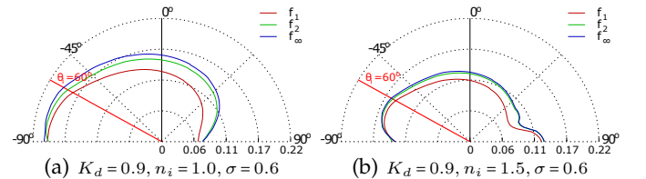
Fig. 9: V-cavities reflectance with inter-reflections, Beckmann distribution: f_1 corresponds to the BRDF with a single light bounce; f_2 corresponds to two light bounces; f_\infty includes all bounces, using a Russian roulette strategy.
