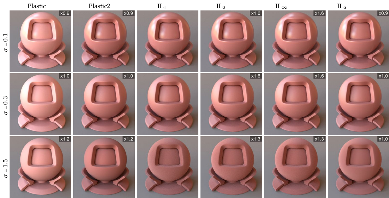
Fig. 16: Comparison between IL and other existing models, with n_i = 1.5 , and \sigma = 0.1 for the first row, \sigma = 0.3 for the second row, \sigma = 1.5 for the third row. The first two models (columns) correspond to a Lambertian term for the body reflection, associated with Cook-Torrance. Plastic has a constant Lambertian value, while Plastic2 uses Kelemen et al. improvement [19]; IL_1 corresponds to IL model; IL_2 adds one reflection bounce between microfacets; IL_\infty includes all reflections; IL_\alpha corresponds to our approximate model. All the model employ a Beckmann distribution associated with Smith GAF except for IL for which Torrance and Sparrow's GAF is used for estimating multiple reflections between microfacets. The reference computation time is given by IL, each other image contains the relative time in the top left corner.
