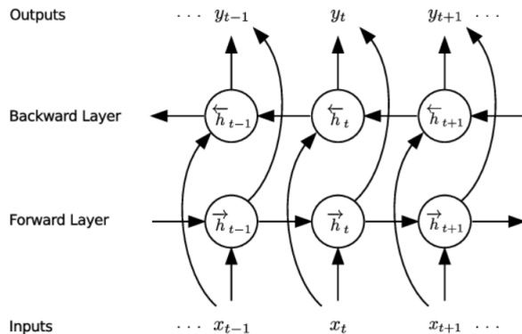
Fig. 1. LSTM model [7]
