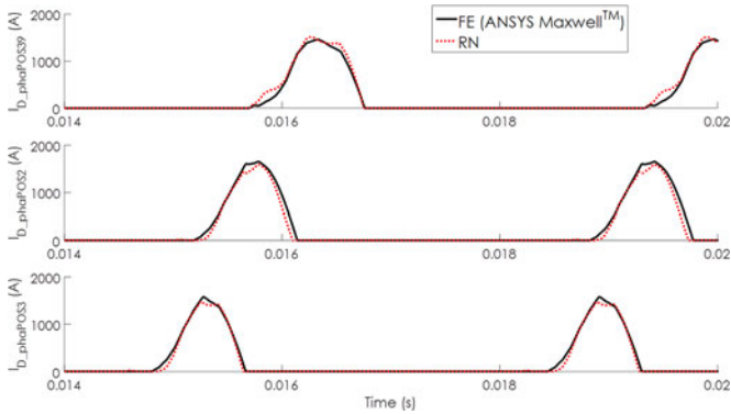
Fig. 25. Comparison of current in diodes of different blocks in fault regime.
