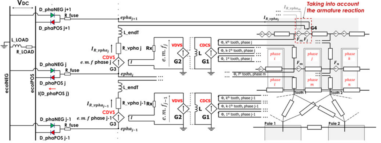
Fig. 11. Coupled circuit model.
