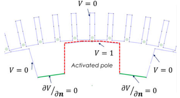
Fig. 6. Application of the boundary conditions.
