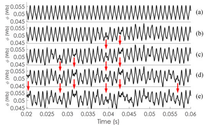
Fig. 31. Flux through sensor coil in healthy case (a), 1 diode opened failure (b), 2 diodes opened failure (c), 3 diodes opened failure (d), and 4 diodes opened failure (e). The time interval of 0.04 s corresponds to a mechanical period with frequency f_m = 25 Hz.
