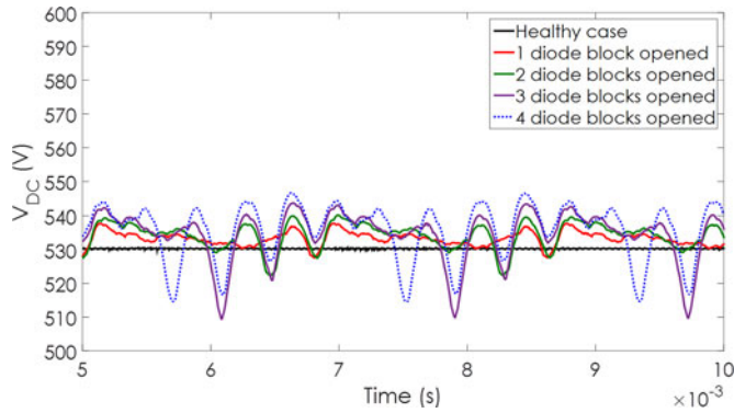
Fig. 28. Simulated rectifier output voltage in open diode fault regimes.
