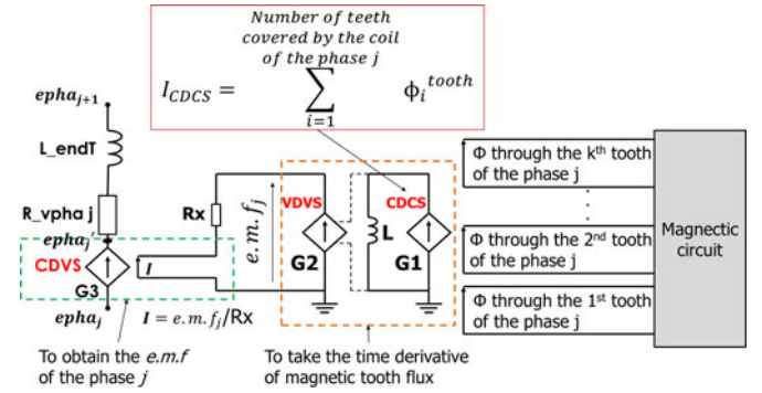
Fig. 10. Coupling circuit used to obtain the phase e.m.f. G1 = 1 , G2 = -N , G3 = Rx , e.m.f. j = -N d\varphi_{total}/dt .
