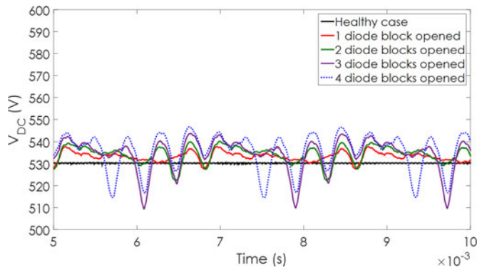
Fig. 28. Simulated rectified output voltage in open diode fault regimes.
