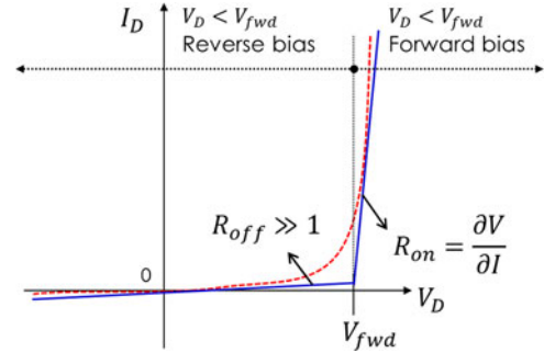
Fig. 12. Diode characteristics.
