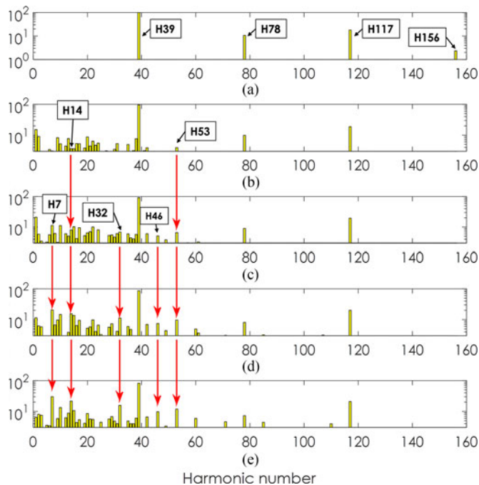
Fig. 32. (a) Spectrum of the sensor flux in healthy case. (b) One diode opened failure. (c) Two diodes opened failure. (d) Three diodes opened failure. (e) Four diodes opened failure. Let us note that the fundamental frequency ( H1 ) corresponds to the mechanical one (25 Hz) and the frequency of the H39 is equal to f_e \times 39/p (975 Hz) where p is the number of pole pairs.
