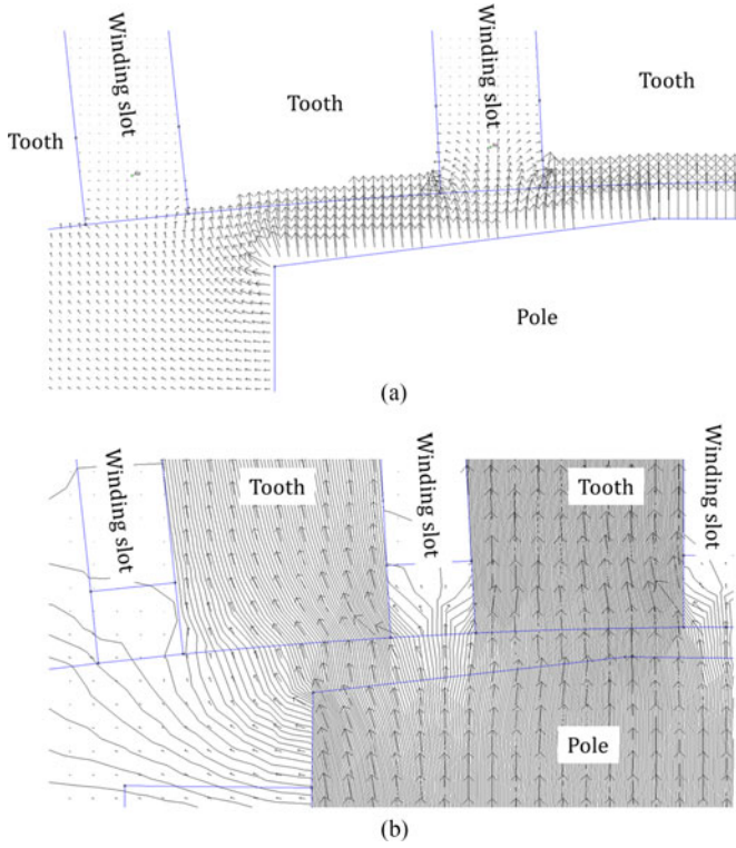
Fig. 7. (a) Distribution of electric induction \vec{D} and (b) magnetic induction \vec{B} .
