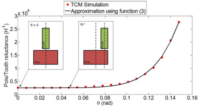
Fig. 8. Evolution of the pole/tooth reluctance as a function of \theta .
