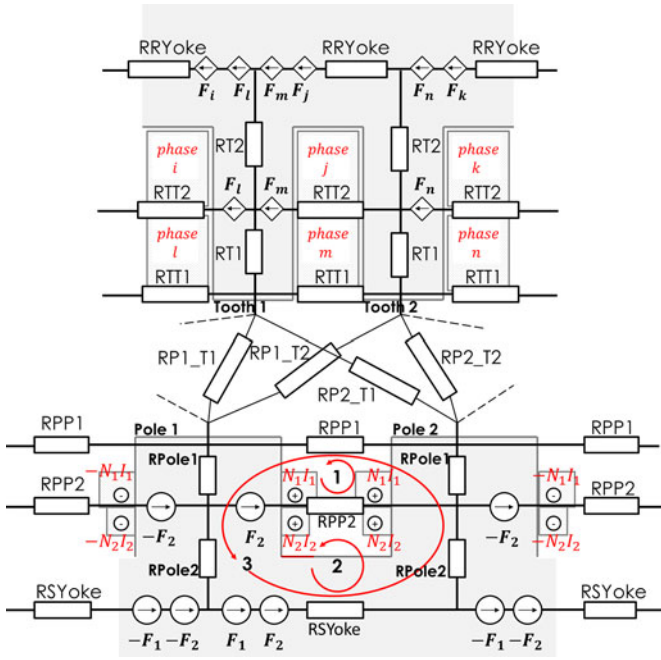
Fig. 4. Portion of the RN showing principal elements.
