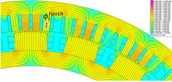
Fig. 13. Simulation result with finite element (FEMM).
