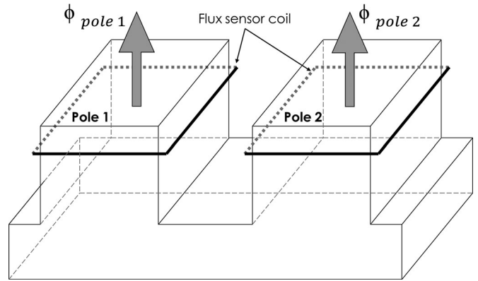
Fig. 30. Flux sensor coils placed on the poles and flux definition associated.
