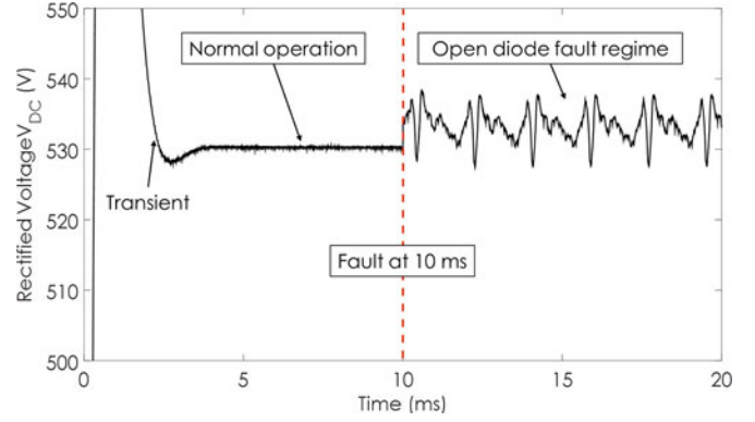
Fig. 21. Simulated rectified voltage by RN model.
