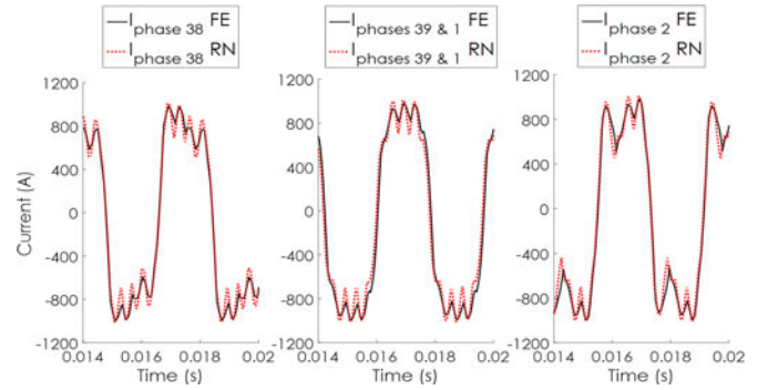
Fig. 23. Comparison of current in different phase coils in fault regime.
