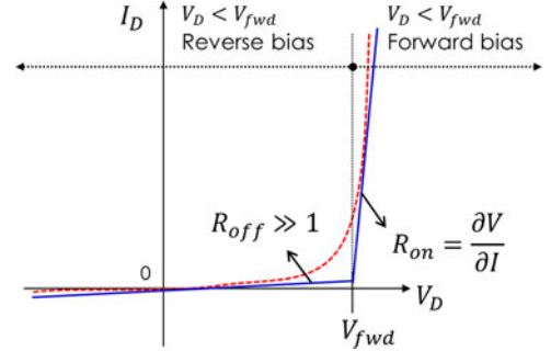
Fig. 12. Diode characteristics.
