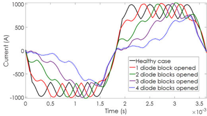
Fig. 29. Phase coil current wave form in healthy case and faulty states. The time interval corresponds to an electrical period ( f_e = 275 Hz).
