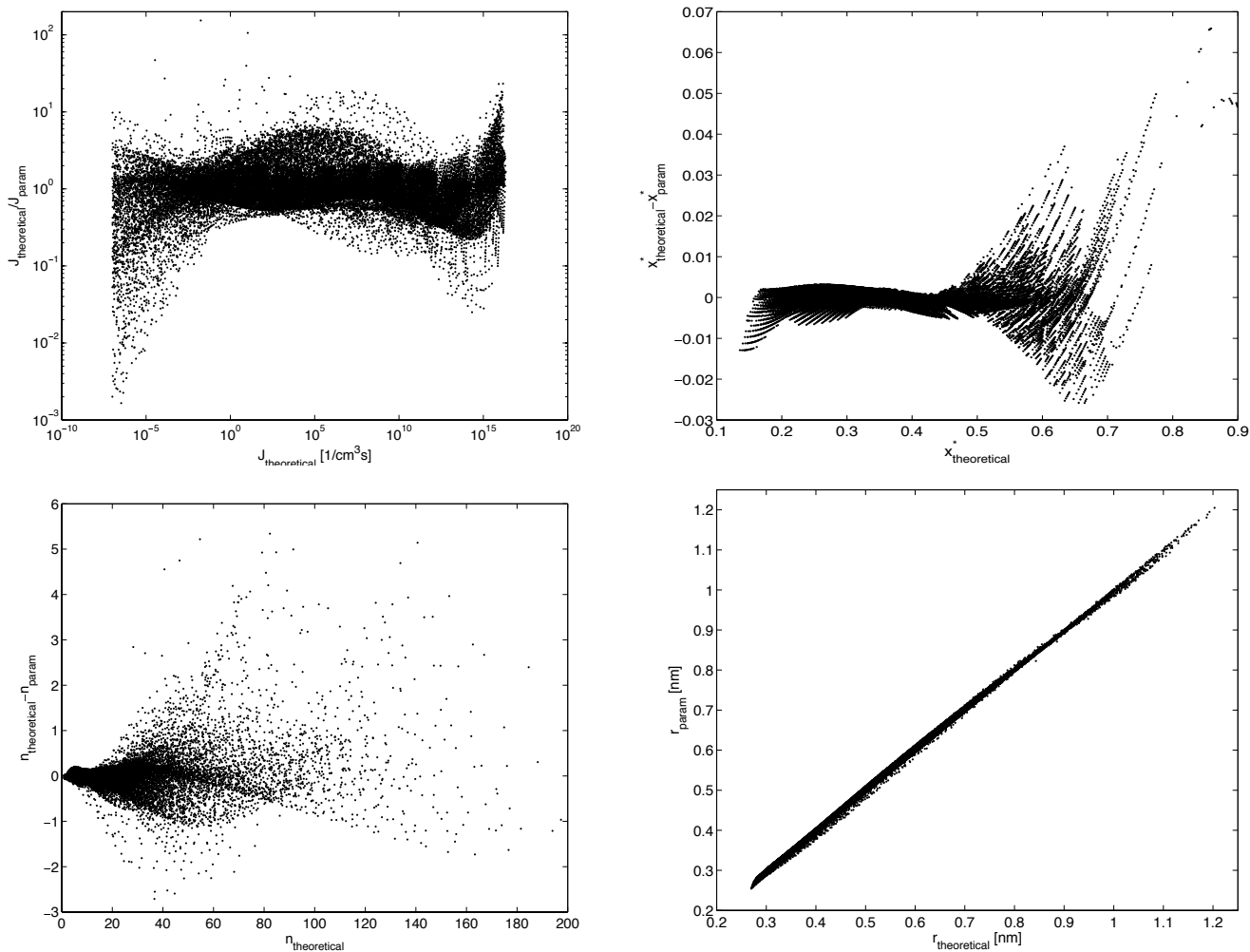
Figure 1. Neutral particle formation: Comparison between the parameterized and the theoretical values for the particle formation rate J (top left), the critical cluster mole fraction x^* (top right), the total number of molecules in the critical cluster n_{\text{tot}}^* (bottom left) and the critical cluster radius r^* (bottom right).
