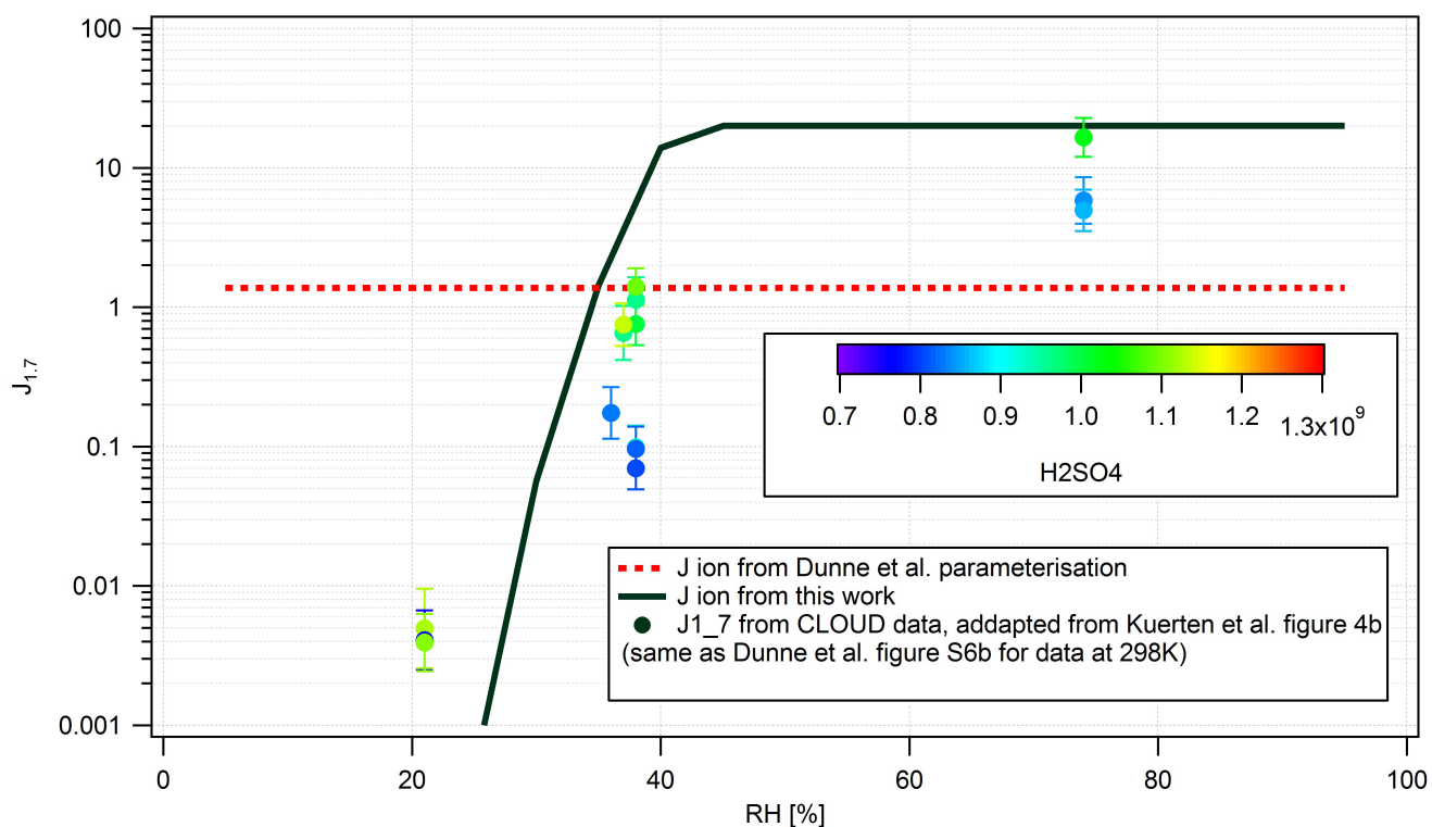
Figure 7. Comparison of particle formation rates as a function of relative humidity given by the parameterization presented in this paper (black solid line, calculated for [H_2SO_4]=10^9 cm^{-3} ), the parameterization of Dunne et al. [2016] (red dotted line) and CLOUD measurements (filled circles with color scale giving the sulfuric acid concentration) for an ion-induced particle formation case at 298 K [see also Figure S6b of Dunne et al. , 2016].
