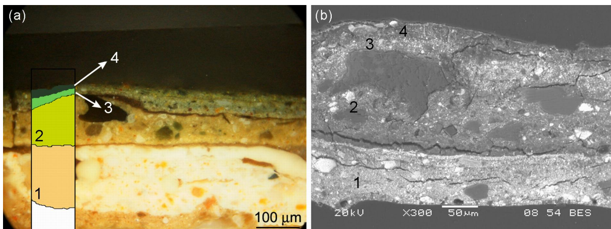
Fig. 3: Cross section with blackened surfaces observed under optical (a) and electron microscope (b) back scattered electrons.
