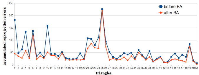
Fig. 3. Accumulated reprojection errors for 52 triangles for a BA applied on the triangle based method estimation
