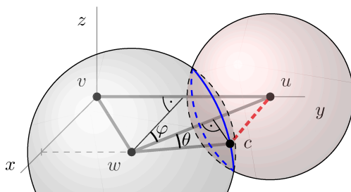
Figure 6: For fixed position of v and w , the angle \varphi determines the position of u , since u lies on the y -axis. If also the length of cw is given, then \theta determines the length of uc . The intersection circle is blue.
