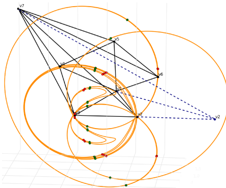
Figure 5: Coupler curve \mathcal{C}_{v_6, \bar{d}} of G_{48} with the edge v_2 v_6 removed. The 28 red points are intersections of \mathcal{C}_{v_6, \bar{d}} with sphere centered at v_2 with edge lengths \bar{d} , whereas the 32 green ones are for edge lengths given by equation (2) (illustrated by blue dashed lines).
