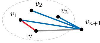
Figure 2: H_{n+1} is constructed by an H1 step applied to H_n (blue edges), extended with the edge uv_{n+1} . This is equivalent with applying an H2 step and adding the deleted edge uv_{n+1} .
