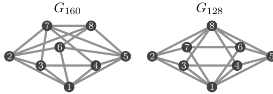
Figure 8: G_{160} has the maximal number of complex embeddings (160). We proved that r_3(G_{128}) = 128 .
