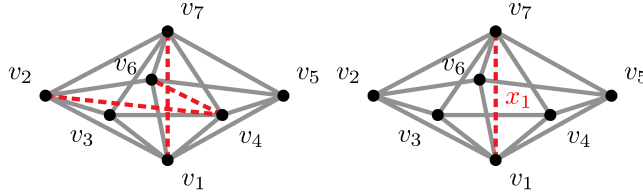
Figure 3: The graph G_{48} (grey edges). There are submatrices of CM_{G_{48}} that involve only variables corresponding to the 3 red dashed edges of the left graph. The graph G_{48} extended by the edge v_1v_7 (that corresponds to the variable x_1 ) is globally rigid.
