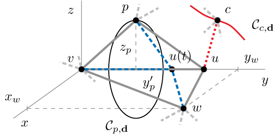
Figure 4: Since the lengths of up and uw are changed accordingly to the length of uv (blue dashed edges), the coupler curves \mathcal{C}_{p,\mathbf{d}'(t)} and \mathcal{C}_{c,\mathbf{d}'(t)} are independent on t . The red dashed edge uc is removed from G .
