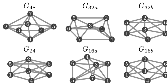
Figure 7: All 7-vertex graphs constructed only by an H2 move in the last step.
