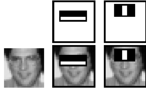
Fig.8. Haar like features (Courtesy of [6])
