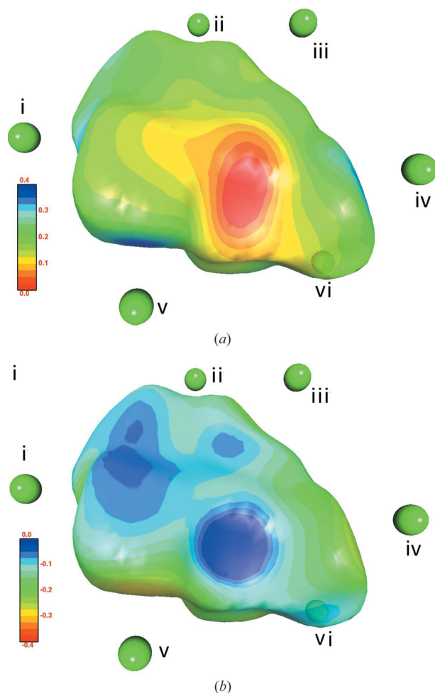
Figure 10 Electrostatic potential on the Hirshfeld surface of the metformin cation. The chloride atoms interacting with the metformin cation are shown. (a) Generated by the cation. (b) Generated by neighboring molecules in contact with the metformin cation. Contributing molecules: chloride ( x, y, z ) and 17 MetCl molecules around the central cation (list given in Table S6). The N3 atom with Lp is in front of the molecule. The closest interacting chloride anions are represented as green spheres and their symmetry number is given: (i) x, y, z ; (ii) -x, y + \frac{1}{2}, -z + \frac{1}{2} ; (iii) x, -y + \frac{1}{2}, z + \frac{1}{2} ; (iv) -x + 1, y + \frac{1}{2}, -z + \frac{1}{2} ; (v) -x + 1, -y + 1, -z + 1 ; (vi) x + 1, -y + 1, z + \frac{1}{2} .
