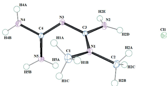
Figure 1 ORTEP view of the MetCl molecule, showing the atom-numbering scheme. Displacement ellipsoids are drawn at the 50% probability level and H atoms are shown as small spheres of arbitrary radii.
