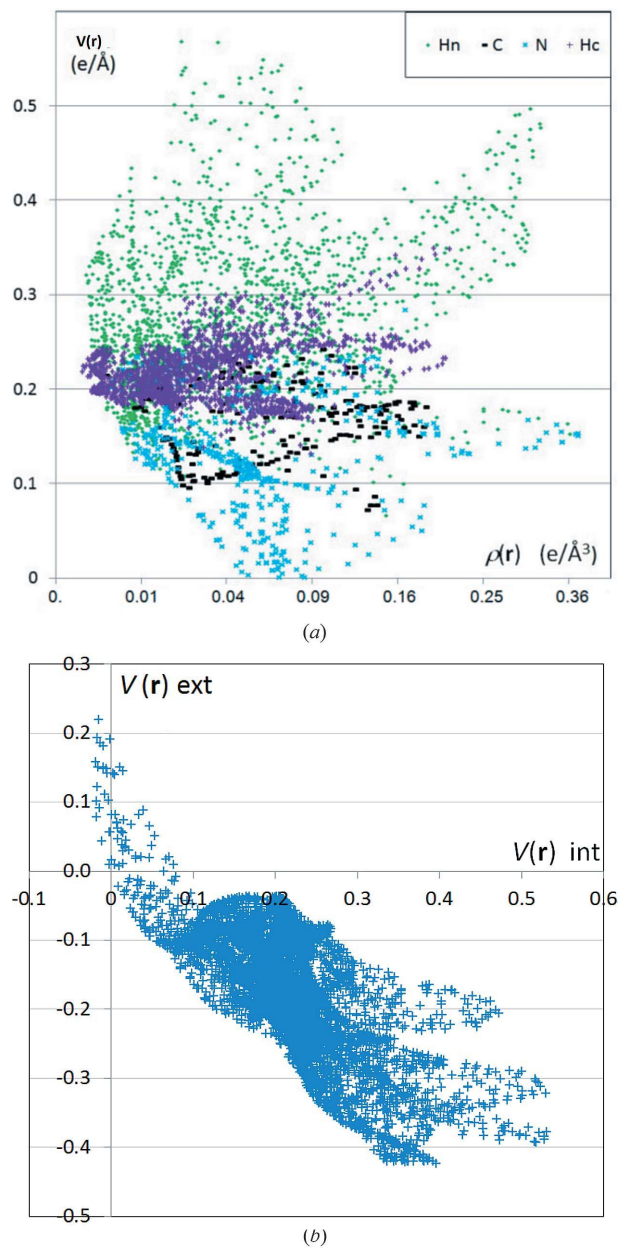
Figure 11 (a) Scatterplot of the electrostatic potential V(\mathbf{r}) generated by the cation versus total electron density \rho(\mathbf{r}) on the Hirshfeld surface around the metformin cation. Notice on the Hirshfeld surface \rho_{\text{ext}}(\mathbf{r}) = \rho_{\text{int}}(\mathbf{r}) . The color indicates the atom type (Hn, Hc, C, N) contributing most to the electron density on the surface. A square-root scale is used for \rho(\mathbf{r}) . The \rho(\mathbf{r}) and V(\mathbf{r}) values on the Hirshfeld surface were retrieved with the software MoProViewer . (b) Scatterplot of the ESP V_{\text{int}}(\mathbf{r}) generated by the cation versus V_{\text{ext}}(\mathbf{r}) generated by the chloride atom of the asymmetric unit plus 17 neighboring MetCl molecules.
