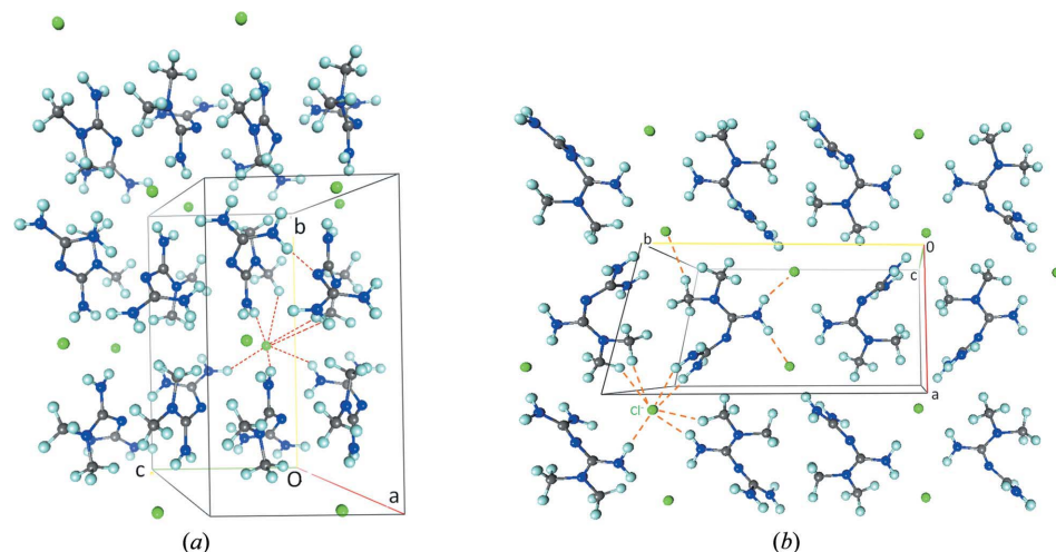
Figure 2 (a) Auto-stereogram showing the crystal packing of MetCl along the a axis. (b) View along the b axis. The Cl...H and N4...H2B hydrogen bonds are shown once in red.
