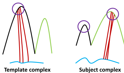
Fig. 1. Two complexes composed of a pseudo cortex, divided into black and green gyri, a blue sub-cortical nucleus and a red fiber bundle. A single diffeomorphism could not put into correspondence all structures and capture the differences in structural connectivity. The points within the violet circle in the template complex would be matched either to the black gyrus of the subject complex or to the red fiber bundle. A double diffeomorphism would first move the fiber bundle from the left to the right gyrus and then it would change the shape of all structures, producing an accurate matching and capturing also the dissimilarities in structural connectivity.
