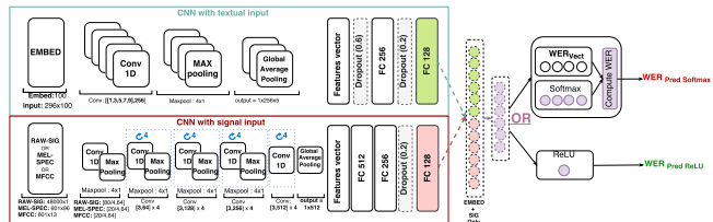
Fig. 1. Architecture of our CNN with text (green) and signal (red) inputs - dotted lines correspond to joint text+signal case
