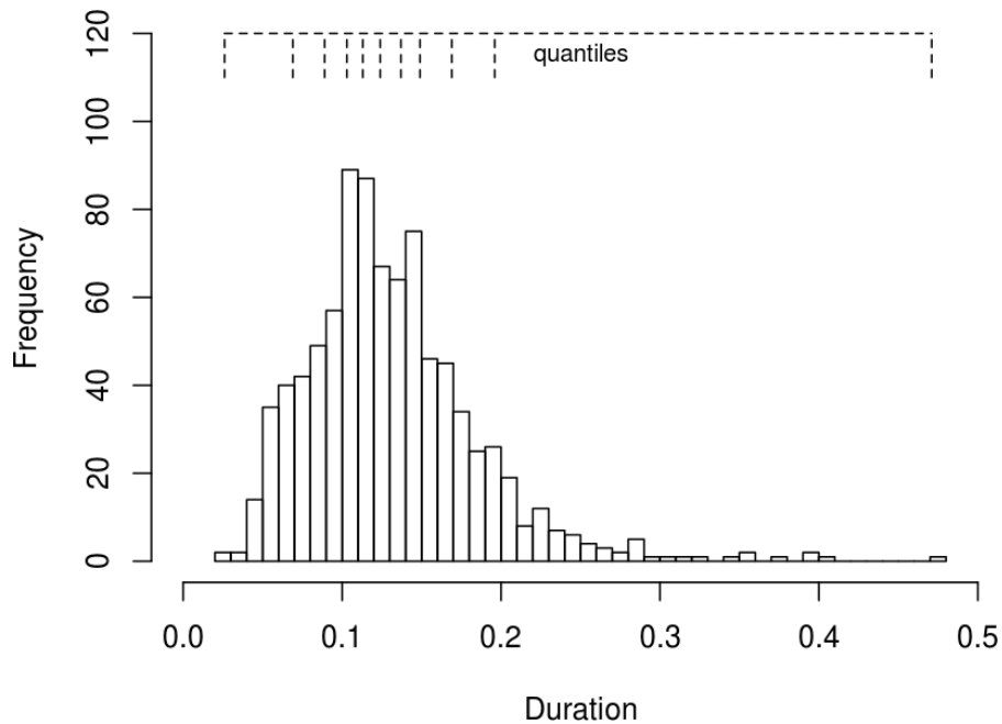
Figure 3a. The distribution of data for the continuous variable DURATION
