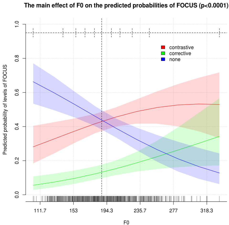
Figure 4. The effect of F0MEAN on FOCUS
