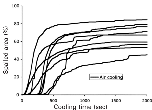
Figure 6 Spallation kinetics of PM2000 oxidised 384 h at 1300°C upon cooling in air-cooled sample-holder.
