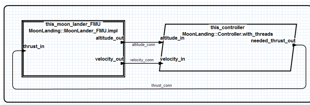
Figure 5 AADL model of the lunar lander
