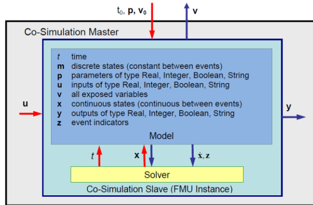
Figure 1 : Data flow between the environment and an FMU for CS [2]
