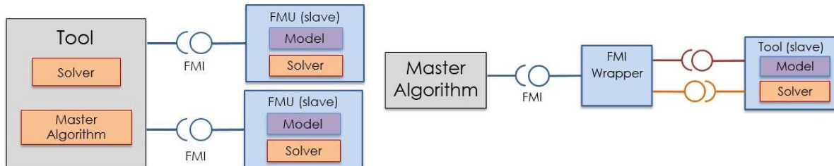
Figure 2: FMU (CS) integration in stand-alone, and with tool coupling [2]
