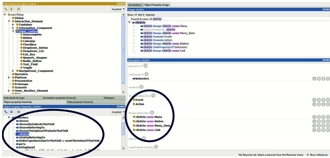
Fig. 5. Ontology structure highlighting the definition of behaviors
