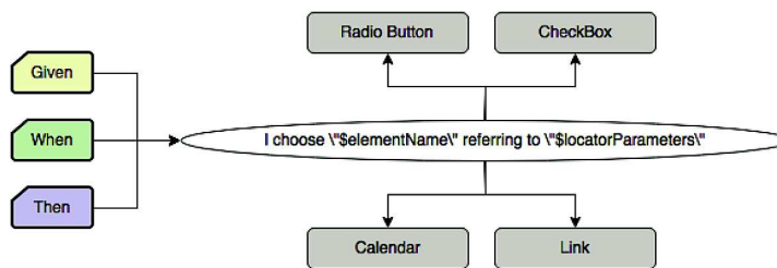
Fig. 6. Behaviors being mapped to UI Elements
